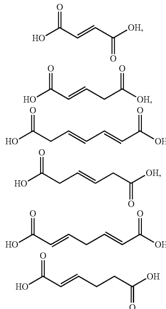
Scheme 1: Straight-Chained Unsaturated Dicarboxylic Acids
