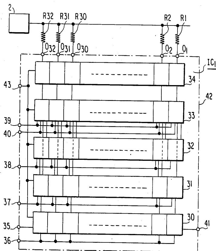
FIG. 2 PRIOR ART
