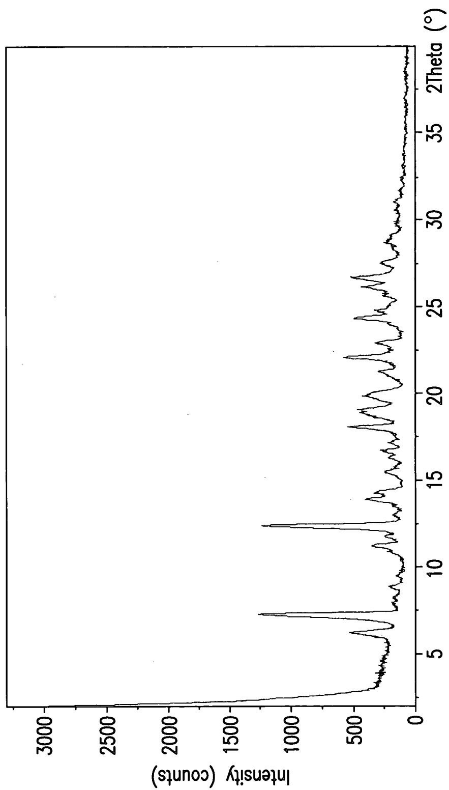
XRPD pattern for the HCl salt polymorphic Form D of Compound I
