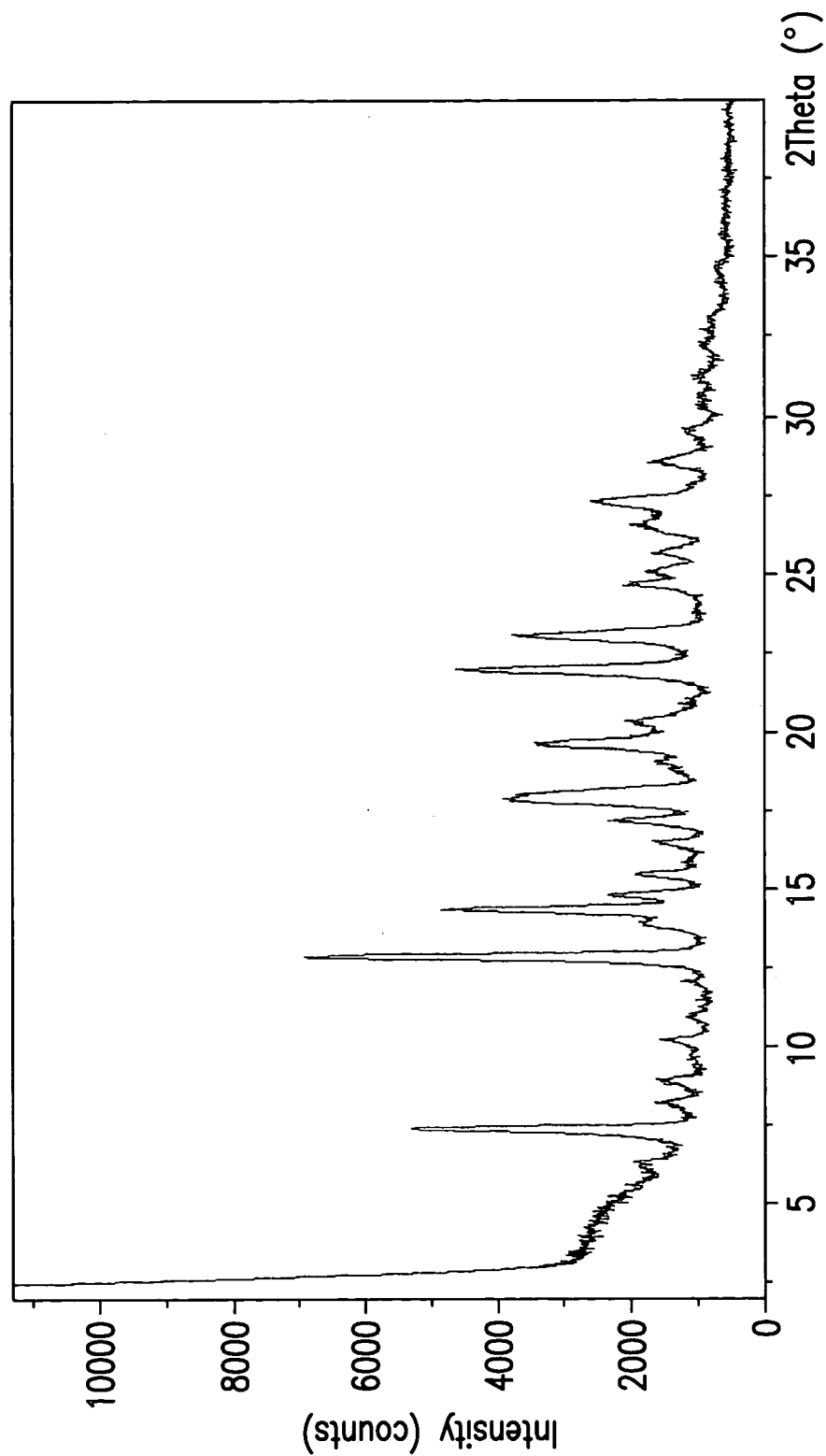
XRPD pattern for the anhydrous HCl salt polymorphic Form E of Compound I
