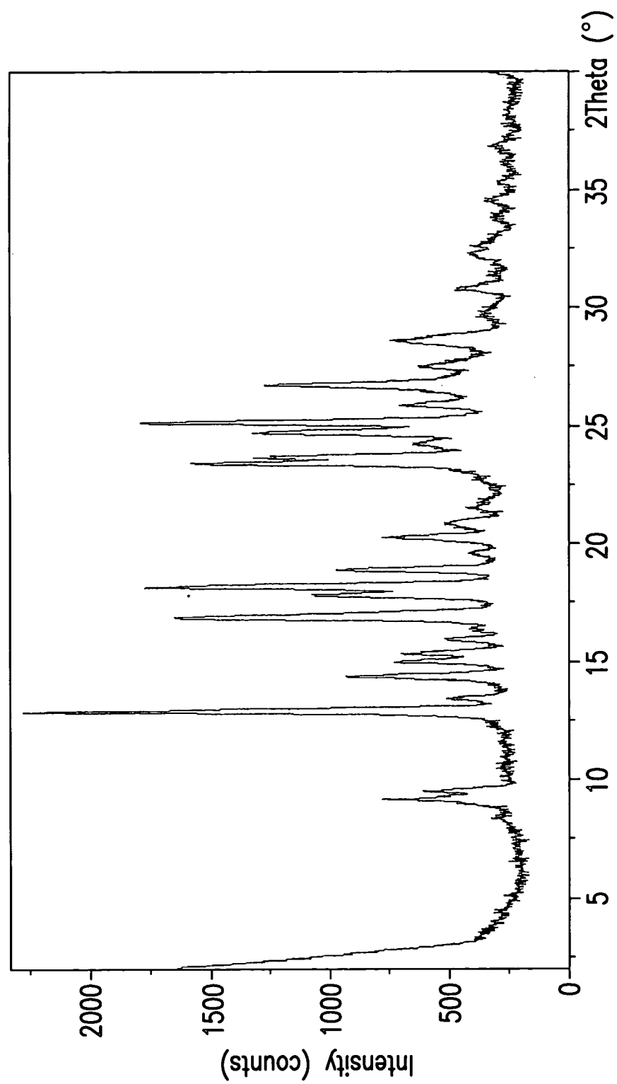
XRPD pattern for the HCl salt polymorphic Form H of Compound I
