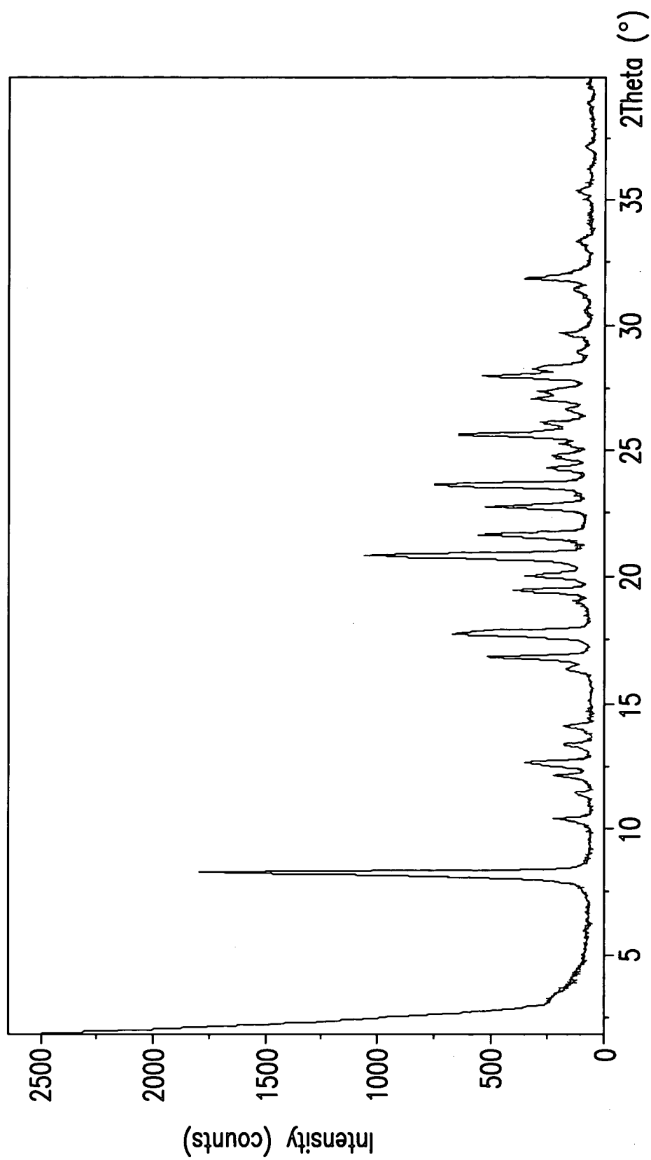
XRPD pattern for the anhydrous HCl salt polymorphic Form G of Compound I
