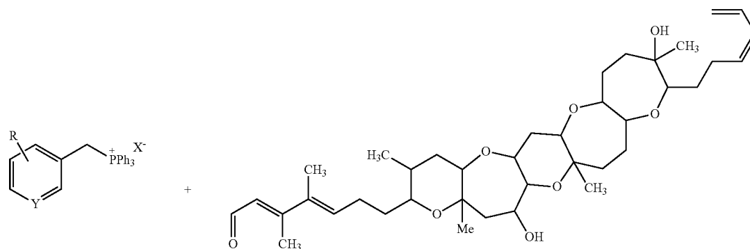
Scheme 5: Synthesis of benzenic derivatives
