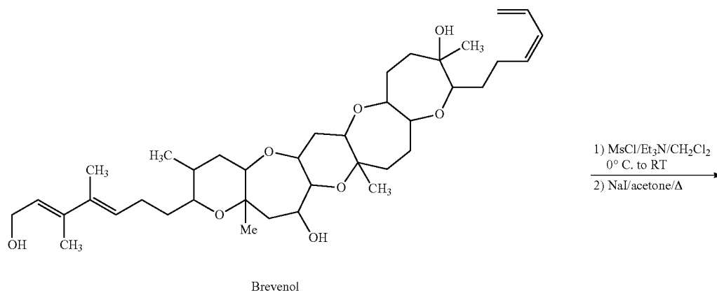
Scheme 6: Synthesis of a benzimidazolone model of brevenol
