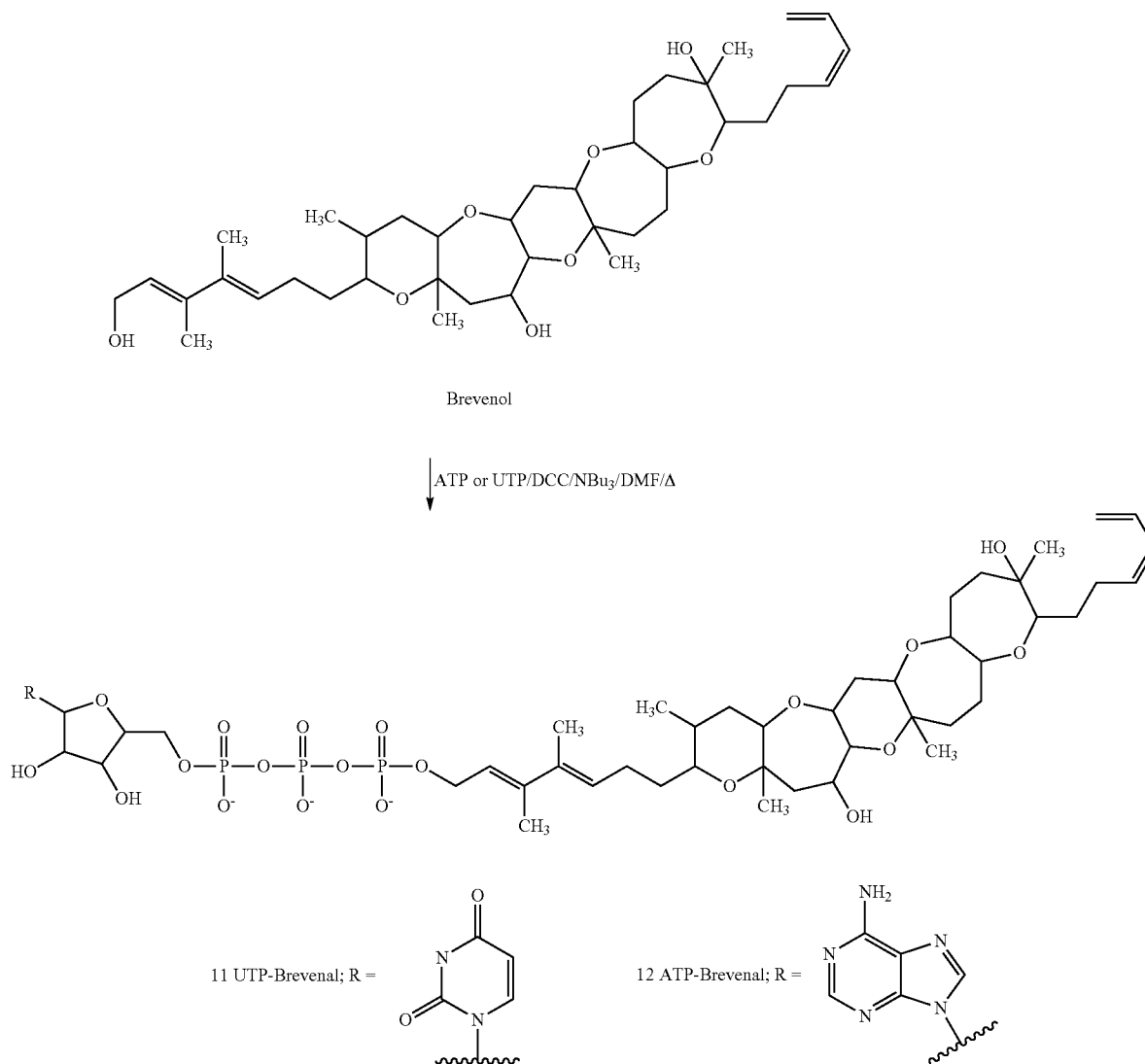
Scheme 7: Synthesis of UTP- and ATP-Brevenal
