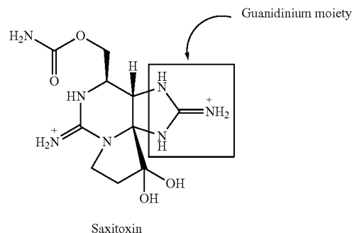
Saxitoxin
