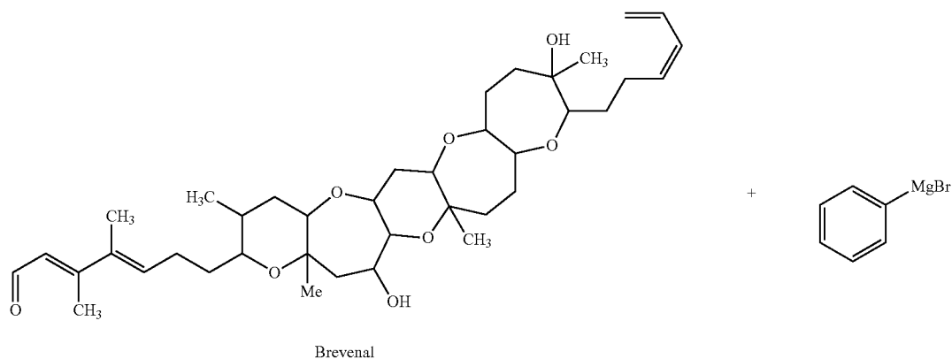
Scheme 4: Synthesis of an ephedrine model of brevenal
