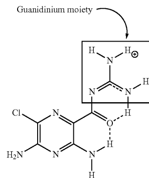
Amiloride structure under physiological conditions
