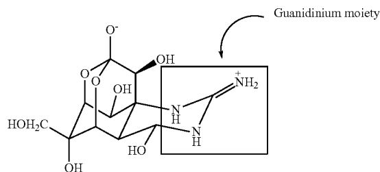
Tetrodotoxin
