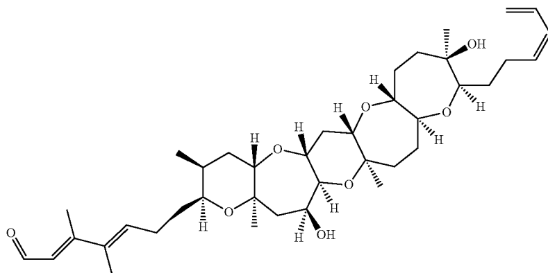
Brevenal
