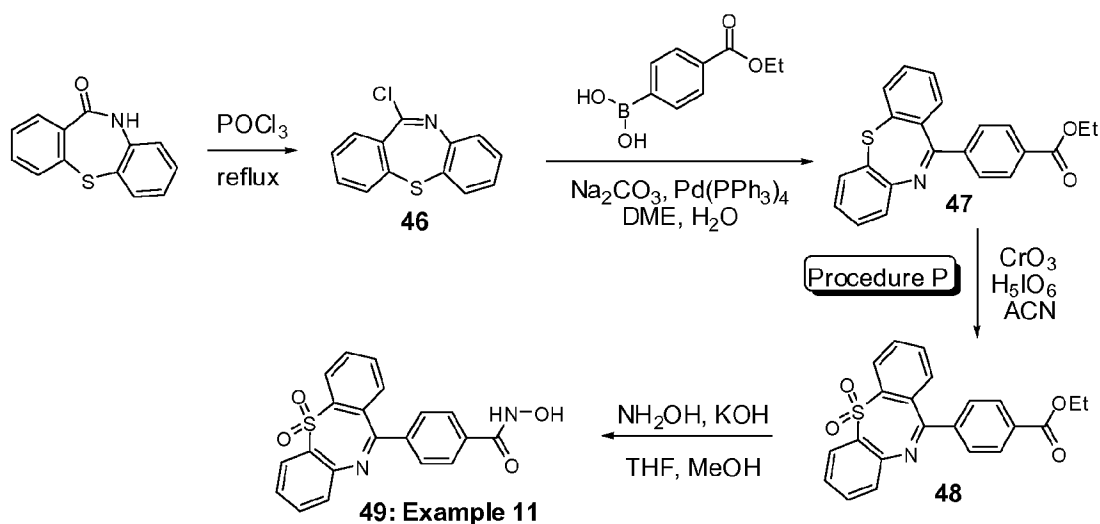
Example 11
