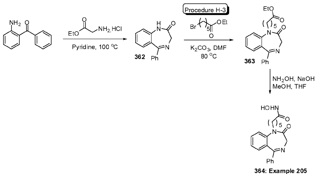
Scheme 55
