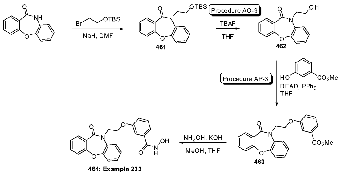
Example 232
