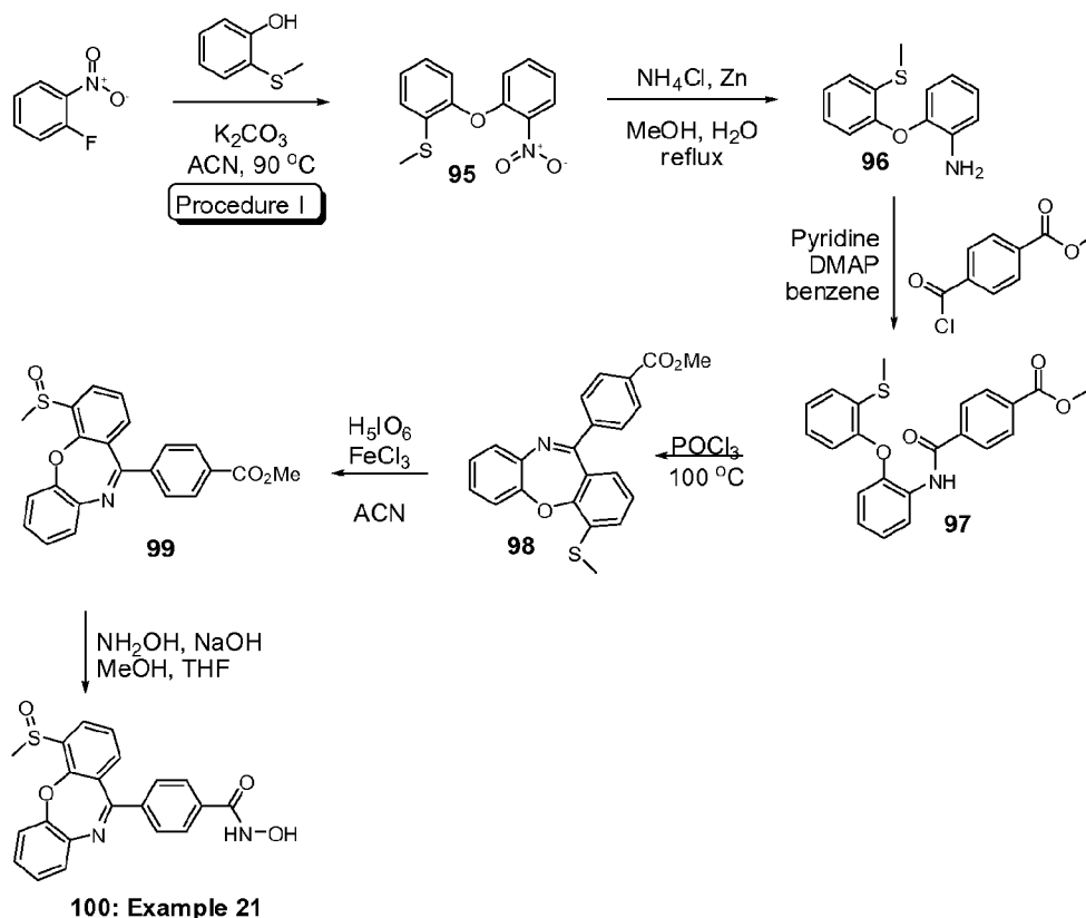
Scheme 20
