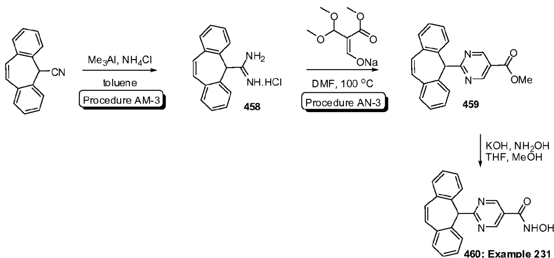
Scheme 81
