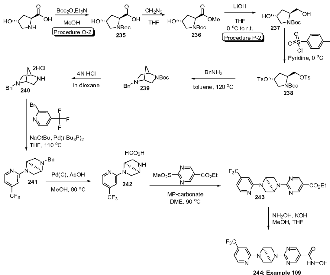
Scheme 39
