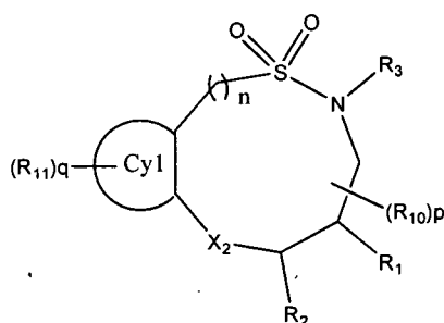
Formula II
