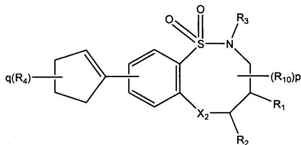
Formula IVA
