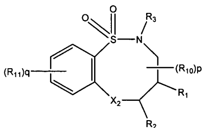
Formula IV
