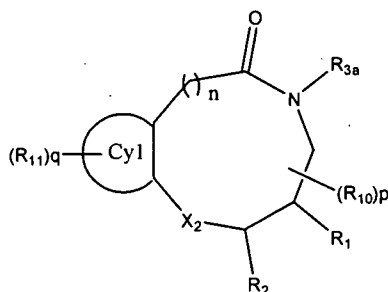
Formula IIIA
