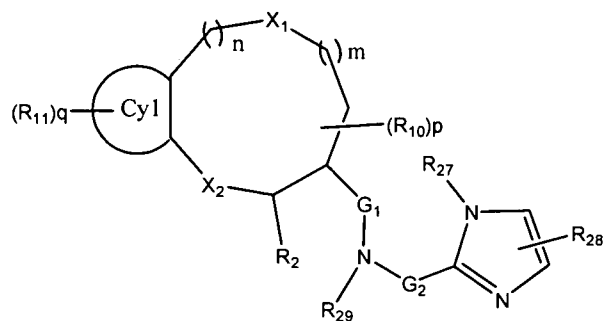
Formula IA
