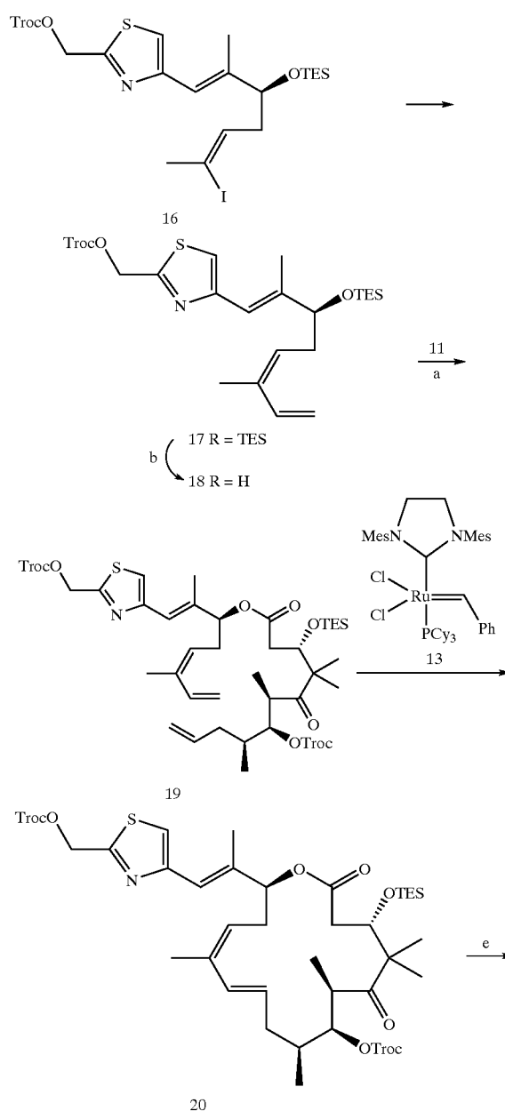
Scheme 2. Synthesis of Compound 4 a
