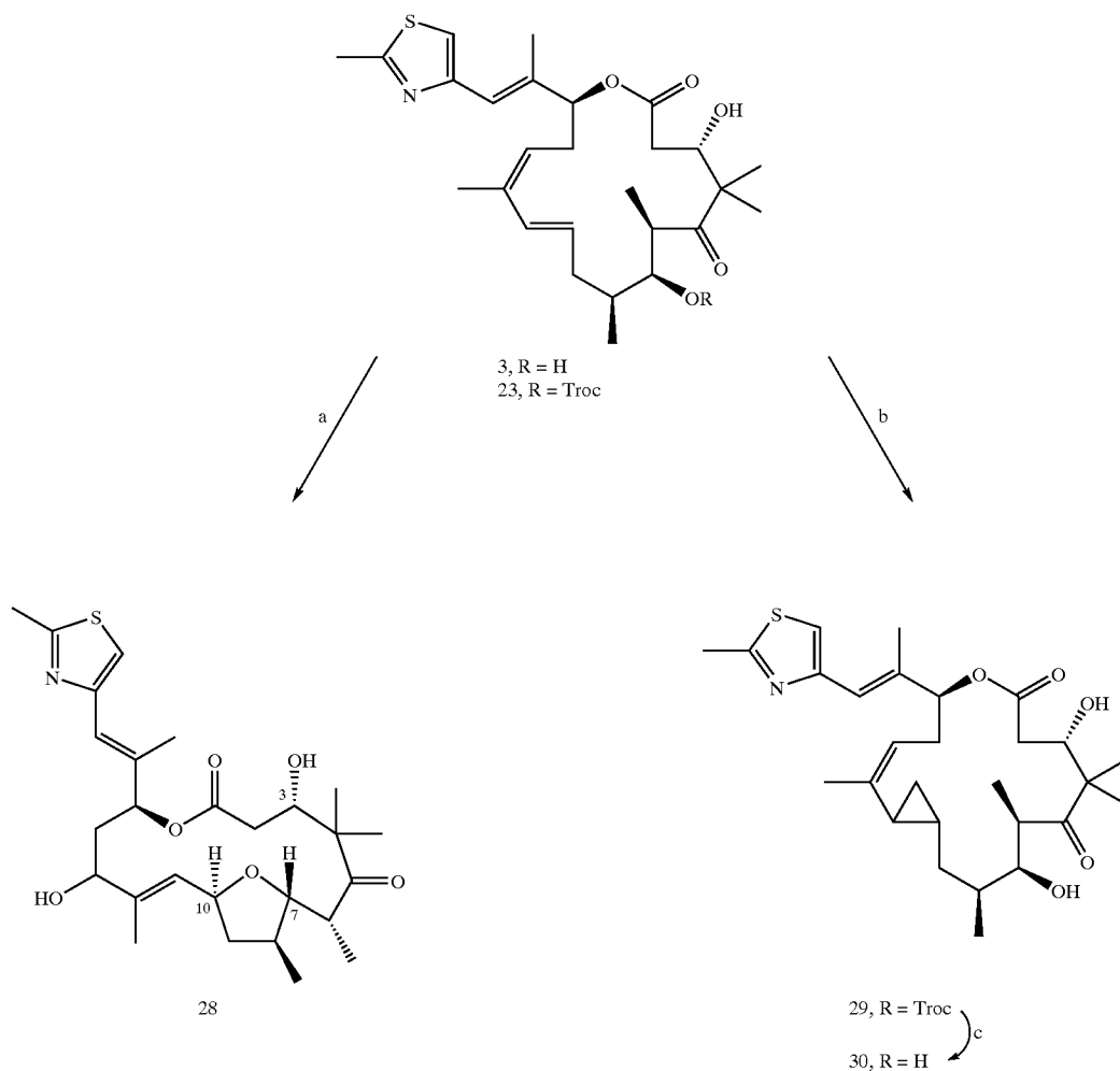
Scheme 6. Selective Epoxidation and Cyclopropanation of Epothilone 490 a
