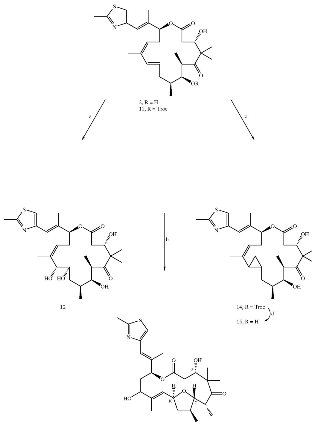
Scheme 3. Selective functionalization of 2 a
