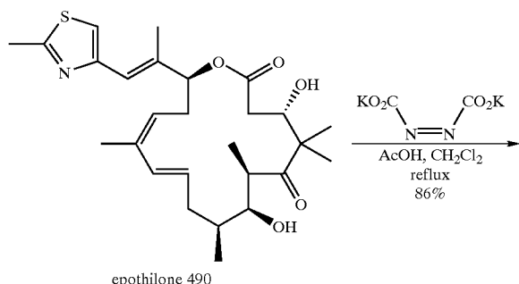
Scheme 4. Diimide reduction of 10,11-Olefin: New Synthesis of dEpoB
