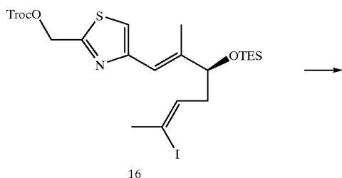
Compounds in Scheme 2:
