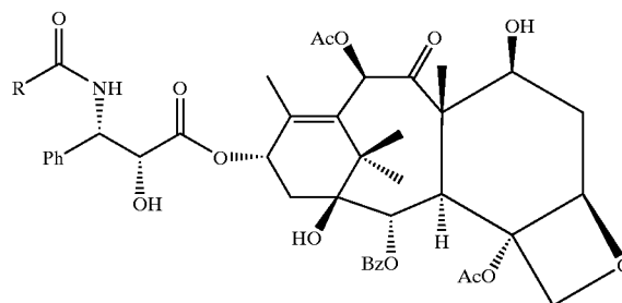
Scheme 1: Taxoids and Epothilones
