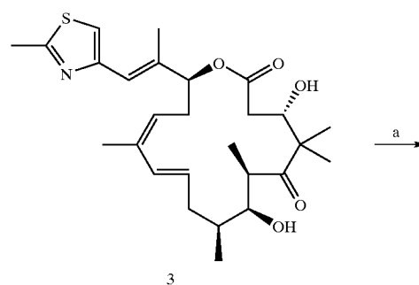
Scheme 5. Selective Dihydroxylation of 10,11-Olefin with OsO 4 a
