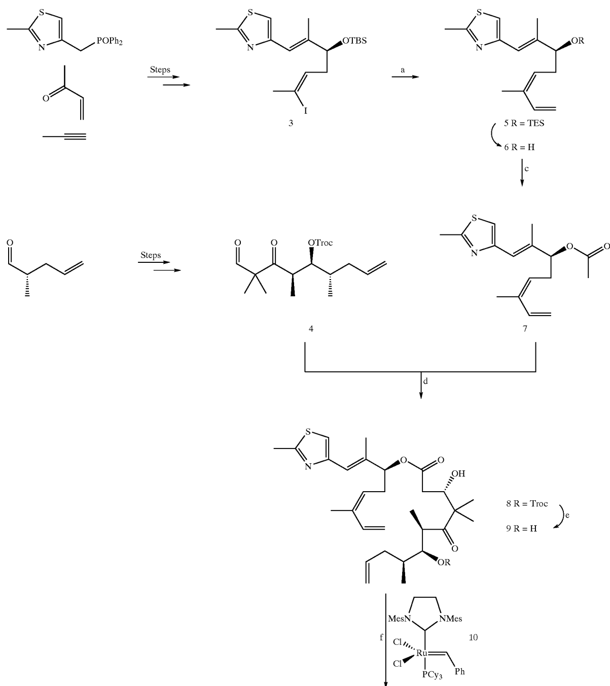
Scheme 1. Synthesis of epothilone 490 a
