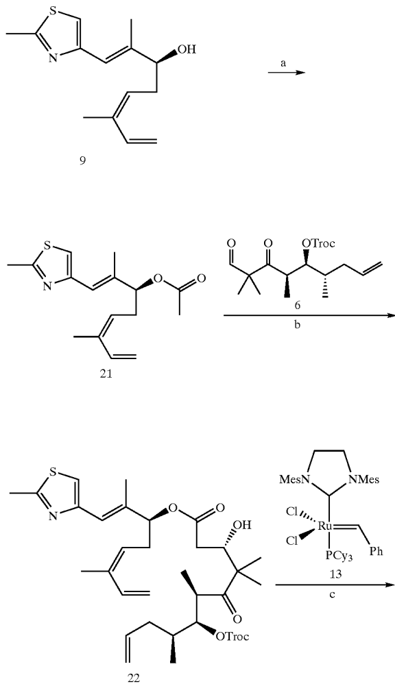
Scheme 3. Epothilone 490 Synthesis via a Late Diastereoselective Aldol Reaction a
