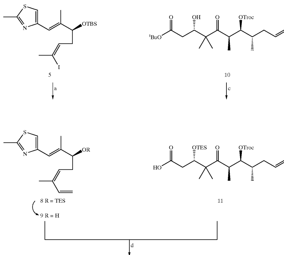
Scheme 1. Initial Ring-Closing Metathesis Route to Epothilone 490 a
