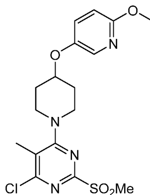
4-Chloro-6-(4-((6-methoxypyridin-3-yl)oxy)piperidin-1-yl)-5-methyl-2-(methylsulfonyl)pyrimidine (Scheme 8)
