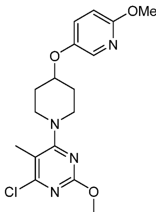
4-Chloro-2-methoxy-6-(4-((6-methoxypyridin-3-yl)oxy)piperidin-1-yl)-5-methylpyrimidine (Scheme 9)
