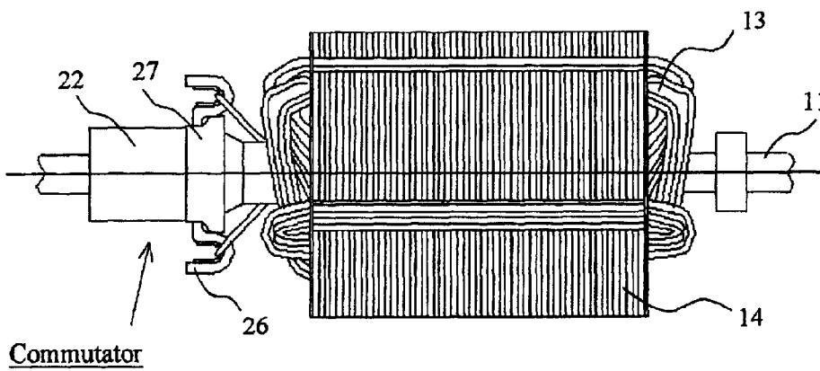
(A) Rotor after Winding and before Spot Welding
