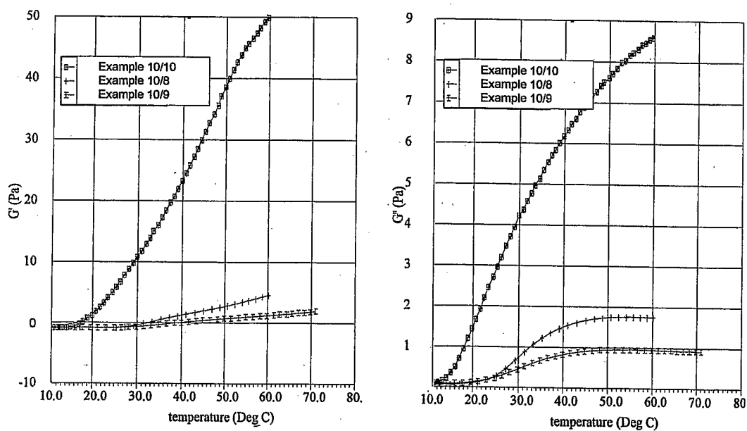
Figure 15: Rheological properties of three-arm star thermo-responsive gels
