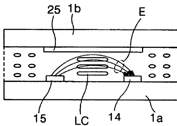
(related art) FIG. 3
