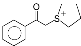
\text{CF}_3(\text{CF}_2)_3\text{SO}_3^- ( z 31)
