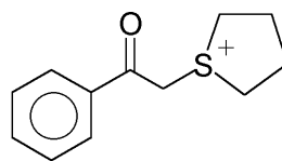
\text{CF}_3(\text{CF}_2)_7\text{SO}_3^- ( z 32)
