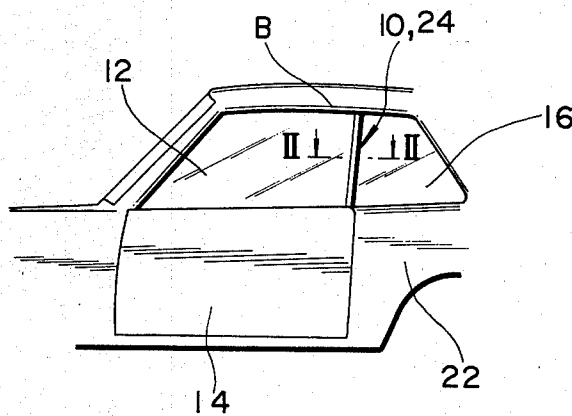
FIG. 2 (PRIOR ART)
