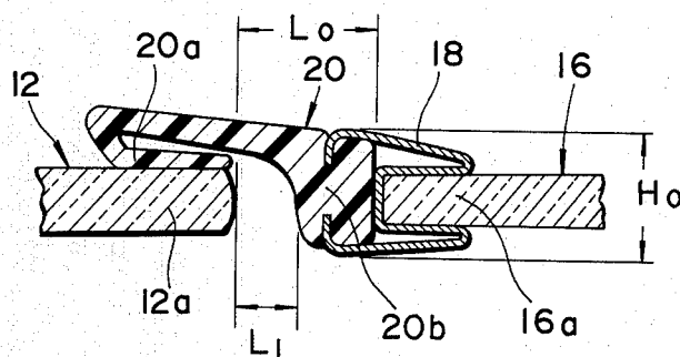
FIG. 2 (PRIOR ART)
