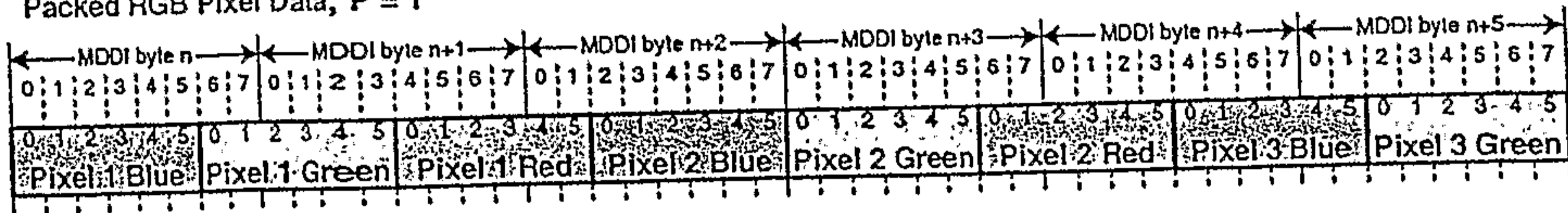
Packed RGB Pixel Data, P = 1
