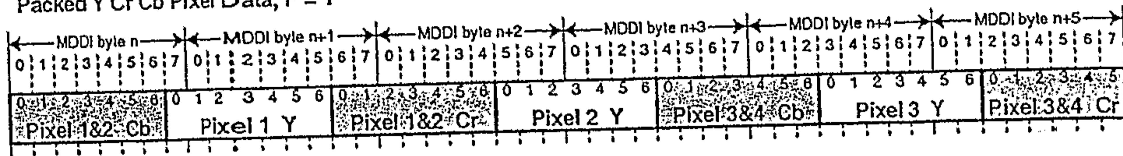
Packed Y Cr Cb Pixel Data, P = 1
