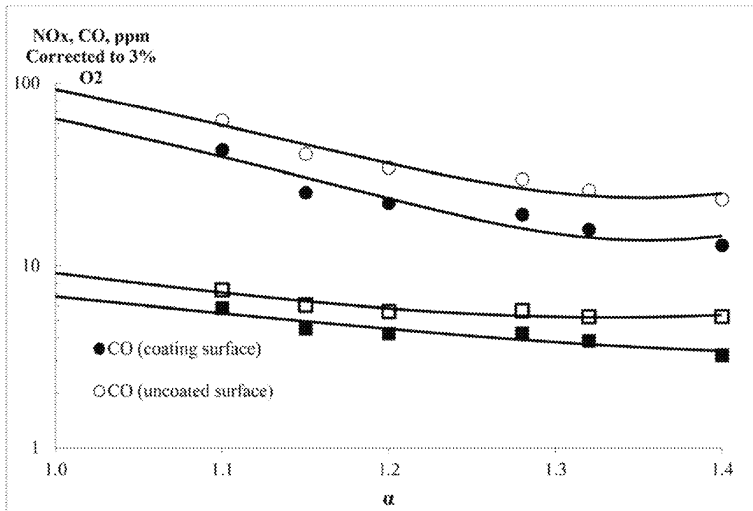
Flue gas CO and NOx corrected concentrations at different excess air ratio (W=33w/cm 2 ).
