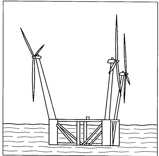
FIG. 4 (PRIOR ART)
