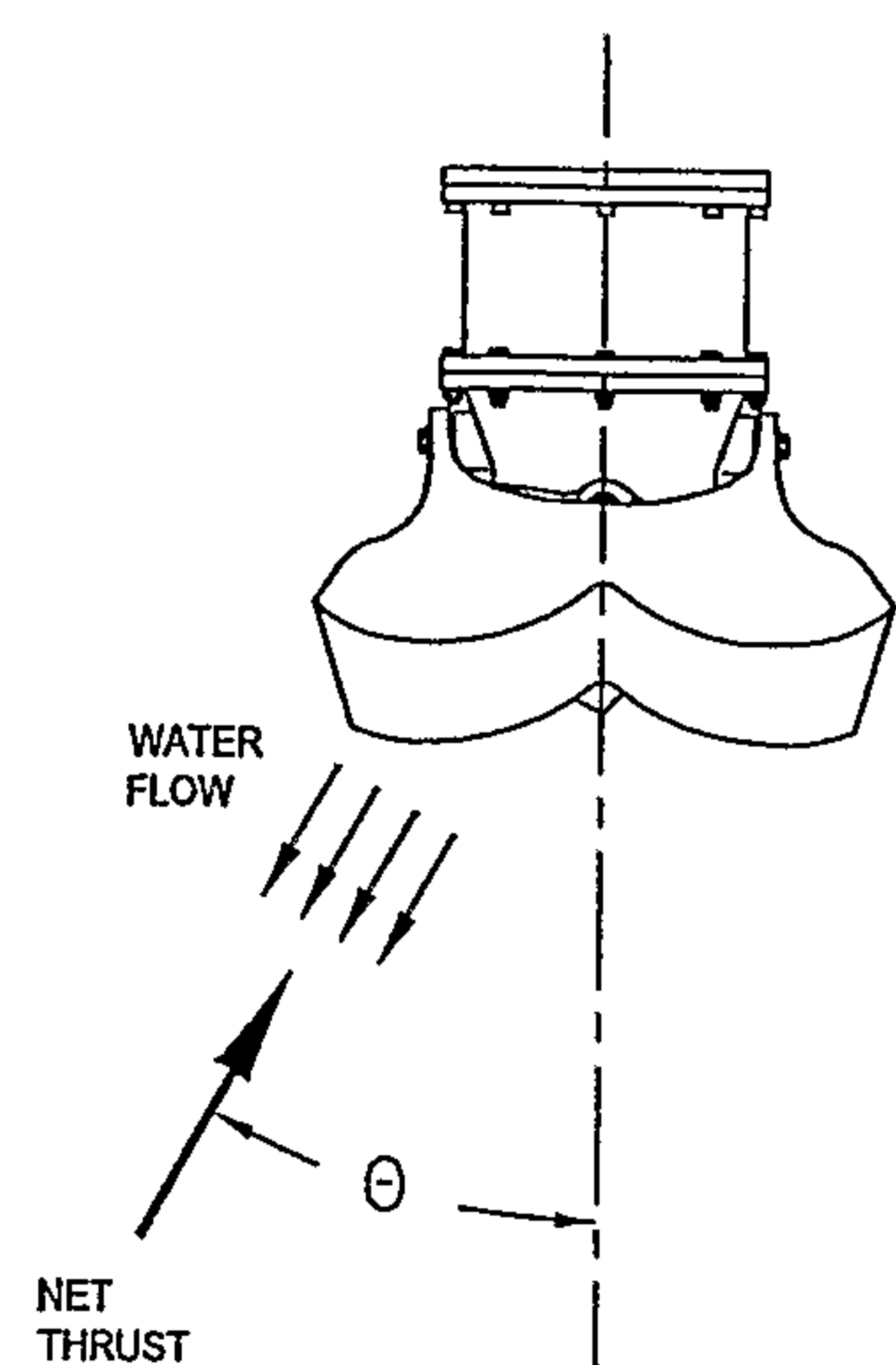
FIGURE 13F HALF THRUST BY MODULATING ENGINE RPM WITH REVERSING BUCKET FULL UP
