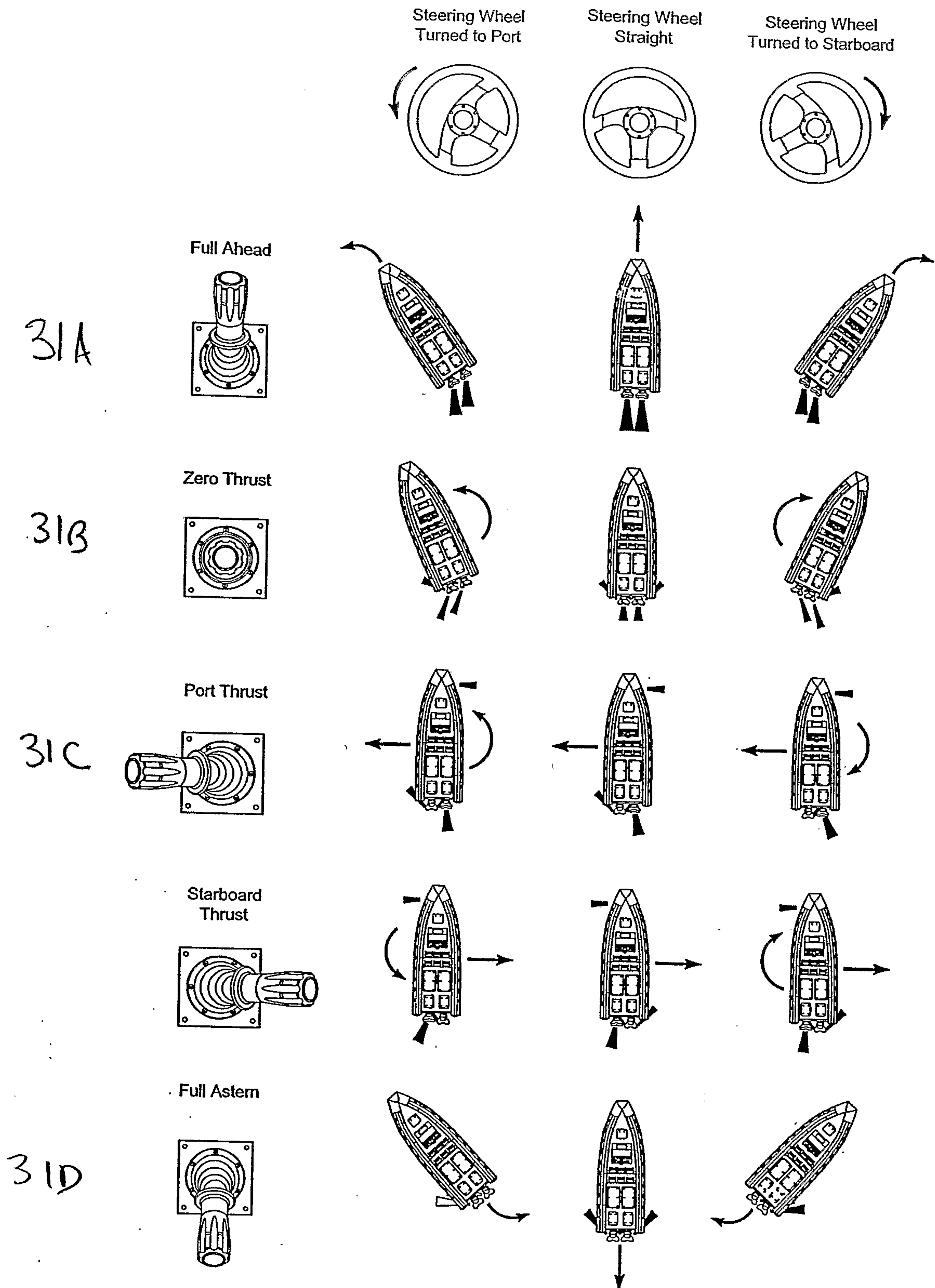
Figure 31 - Vector Stick Dual Water Jet & Bow Thruster Thrust Vector Diagram
