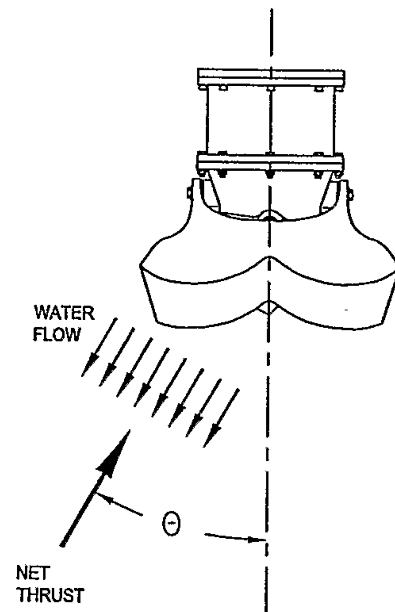
FIGURE 13E FULL THRUST WITH REVERSING BUCKET AT FULL UP
