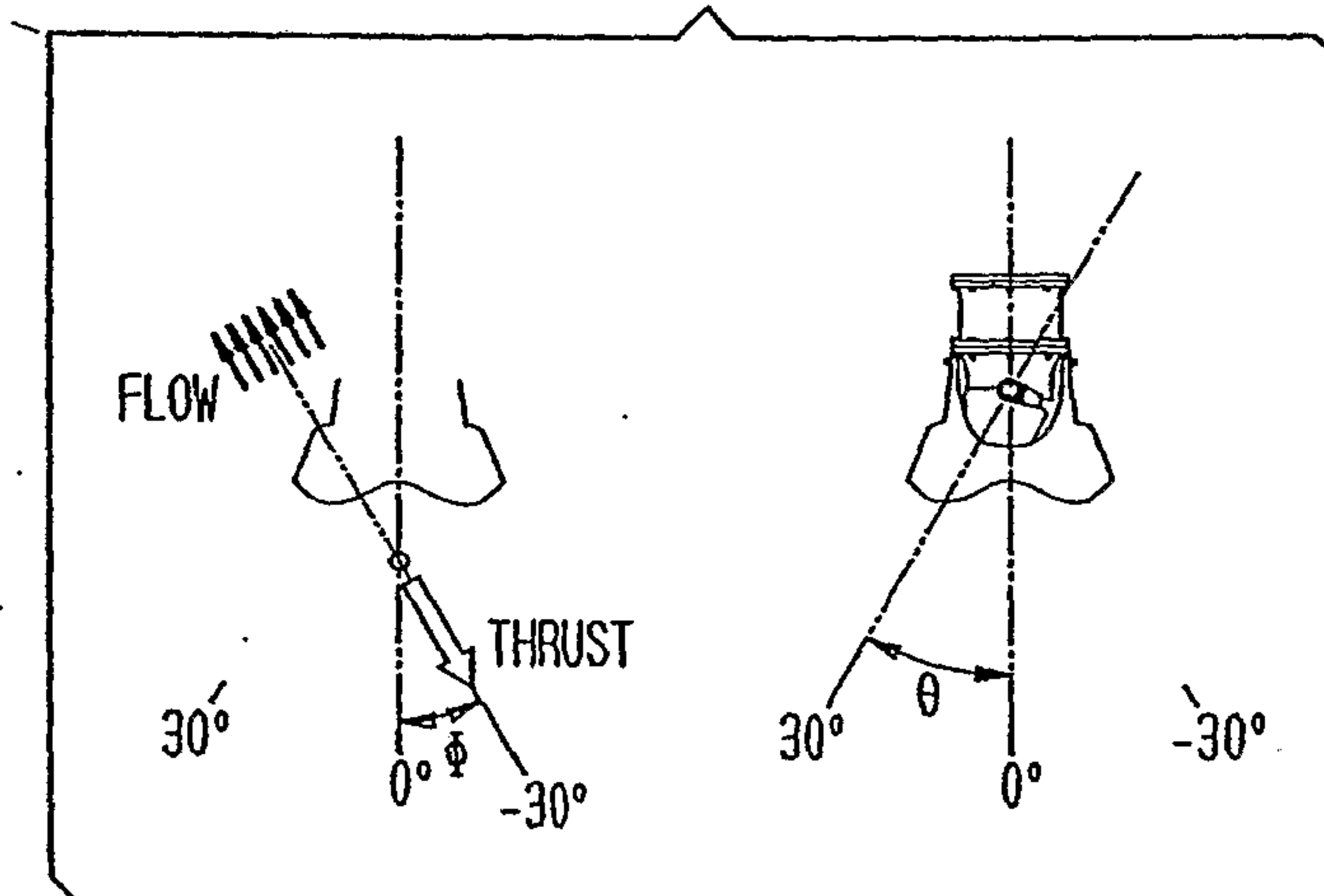
FIG. 25B FULL REVERSE BUCKET
