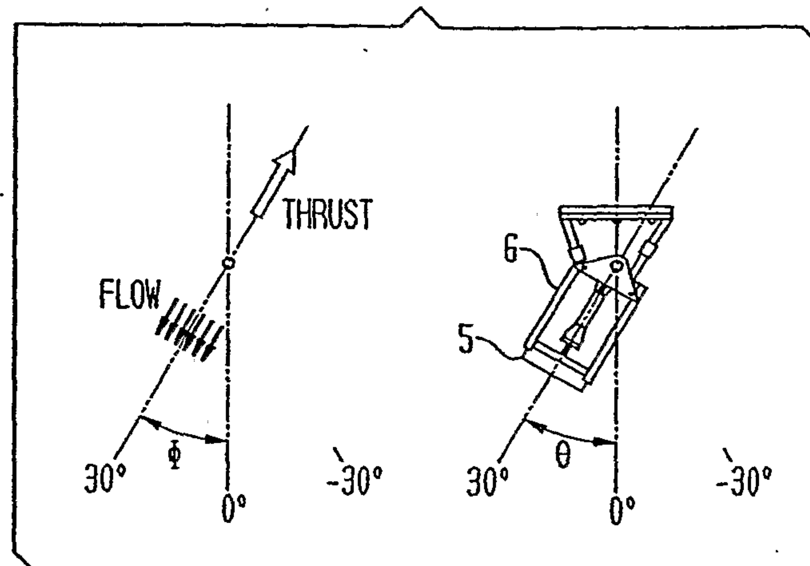
FIG. 22A FULL AHEAD BUCKET
