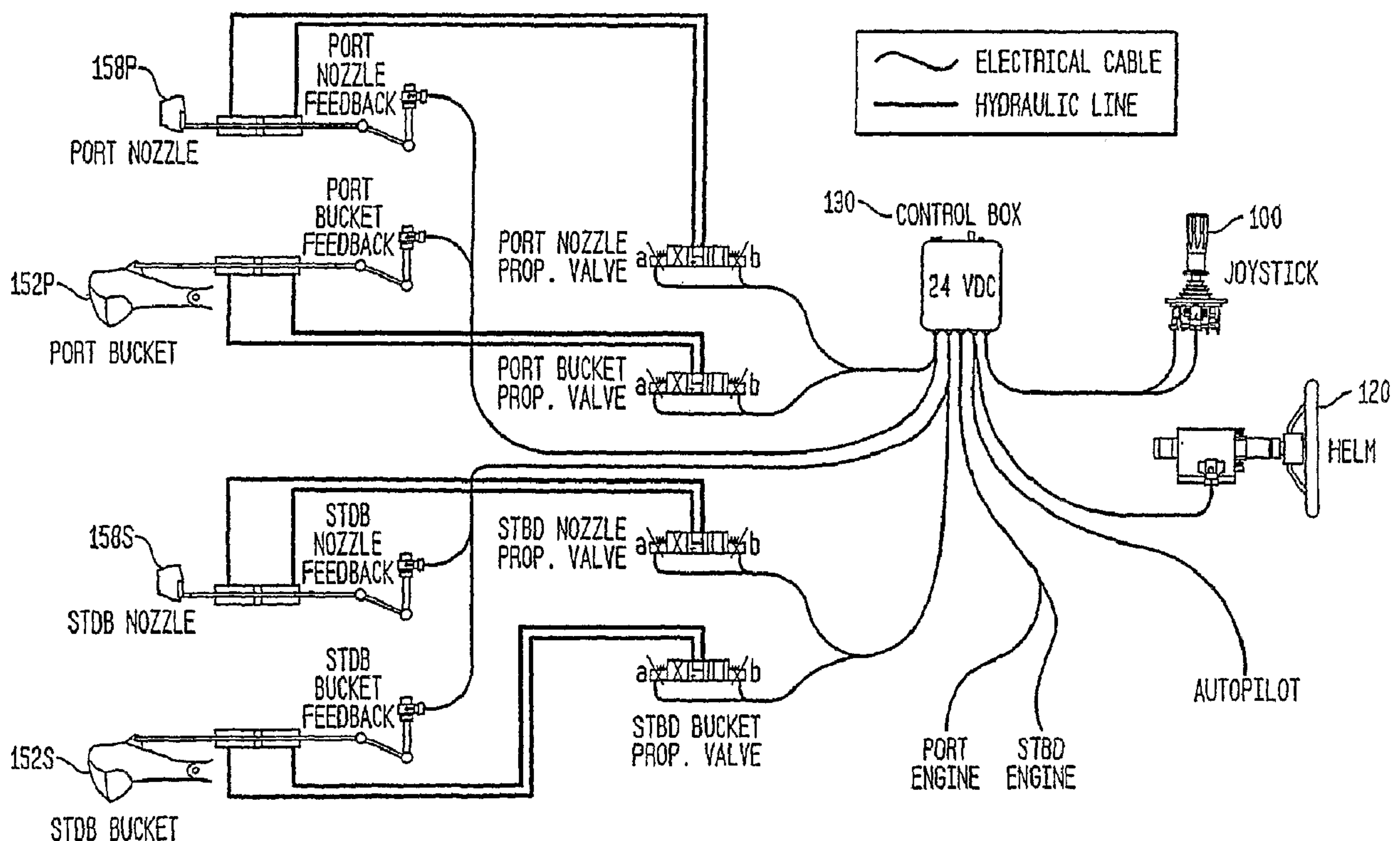
TWIN JET SYSTEM DIAGRAM
