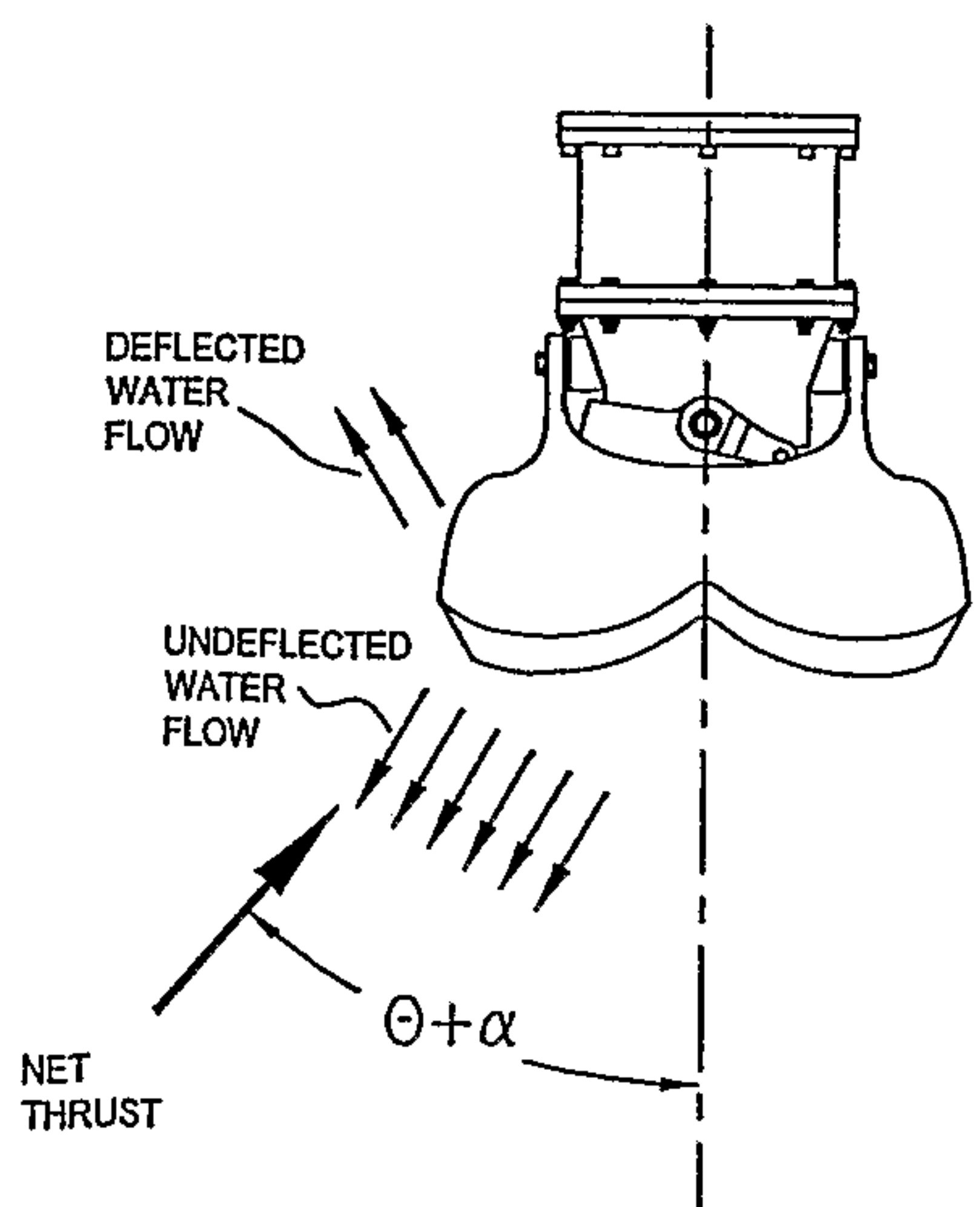
FIGURE 13D HALF THRUST BY MODULATING THE REVERSING BUCKET
