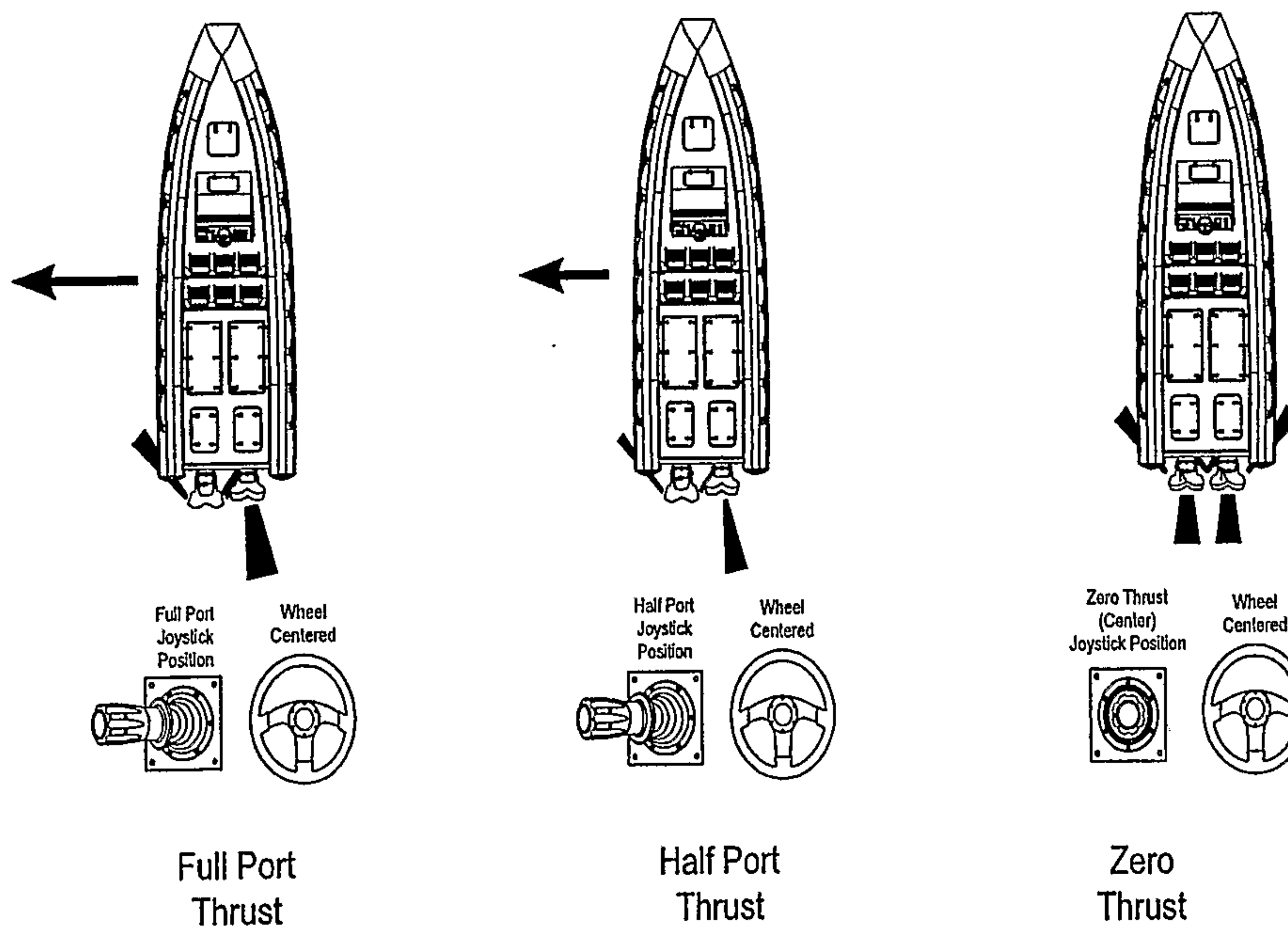
Figure 13H Zero, Half & Full Port Thrust Using Engine RPM Modulation Only
