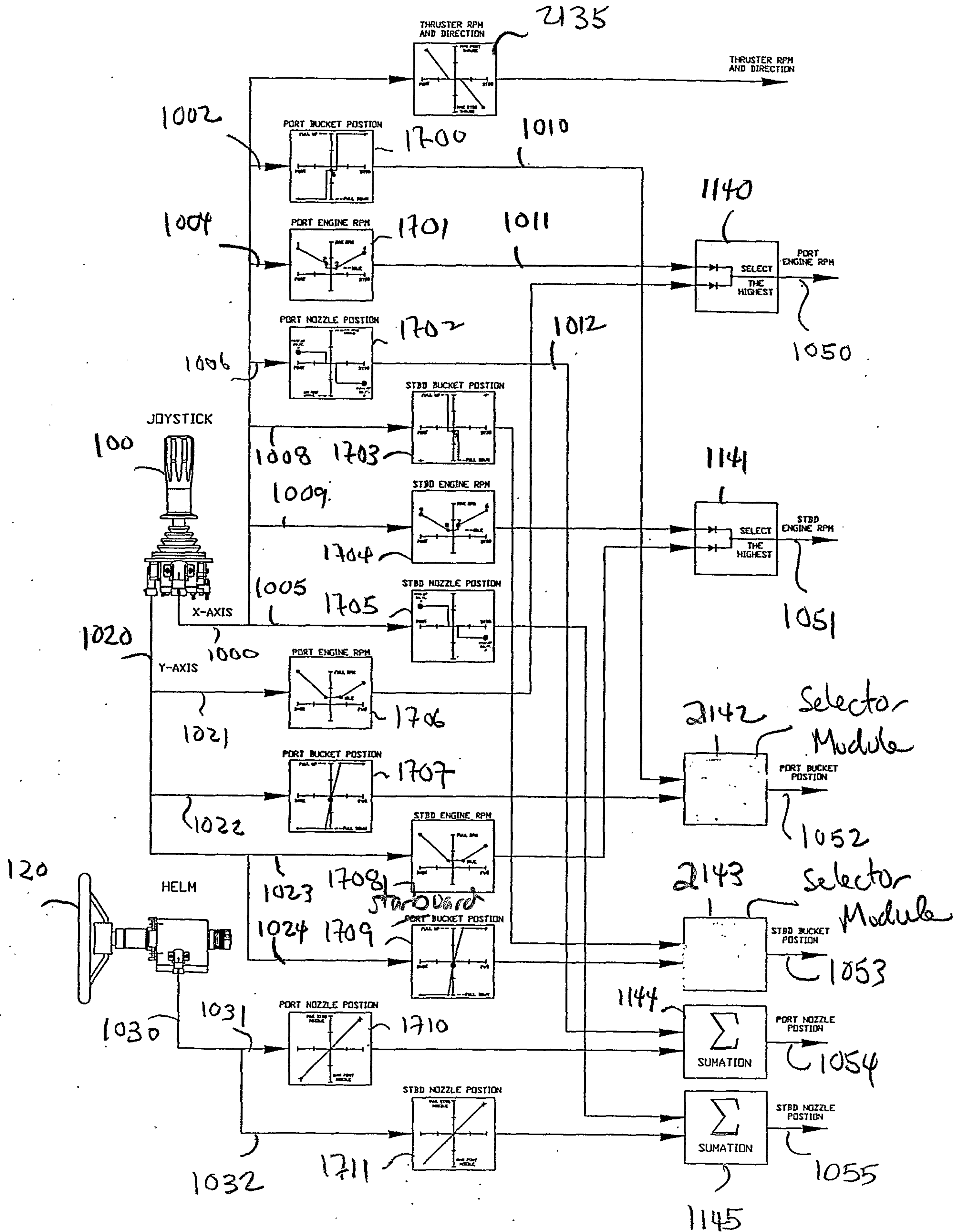
FIGURE 30 - TWIN WATERJET SIGNAL DIAGRAM WITH BOWTHRUSTER
