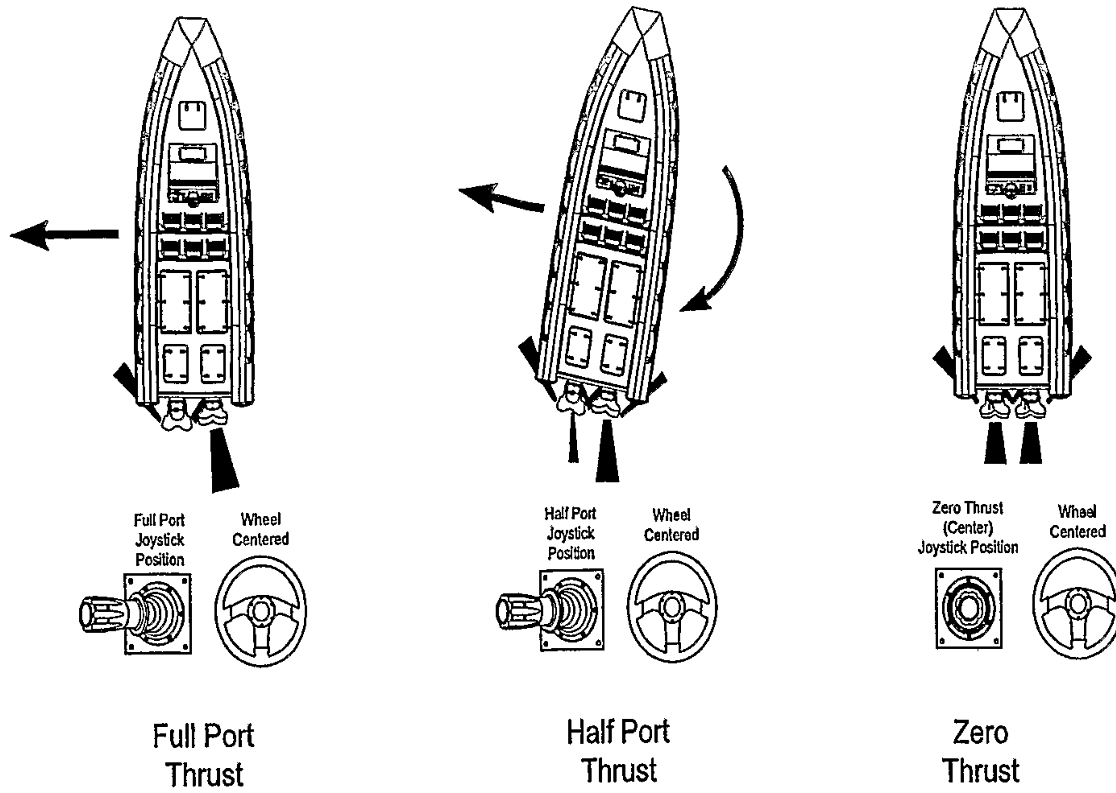
Figure 13G Zero, Half & Full Port Thrust Using Reversing Bucket Modulation
