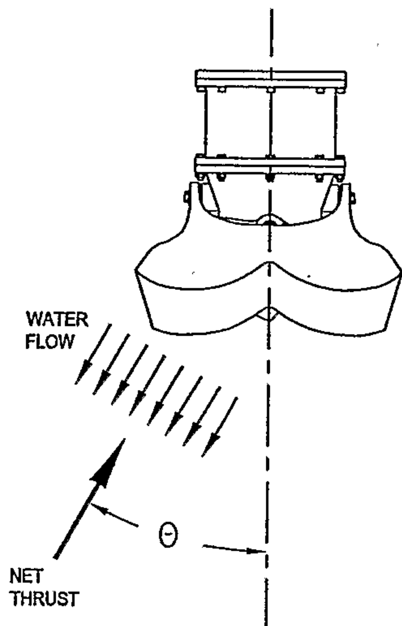
FIGURE 13C FULL THRUST WITH REVERSING BUCKET AT FULL UP
