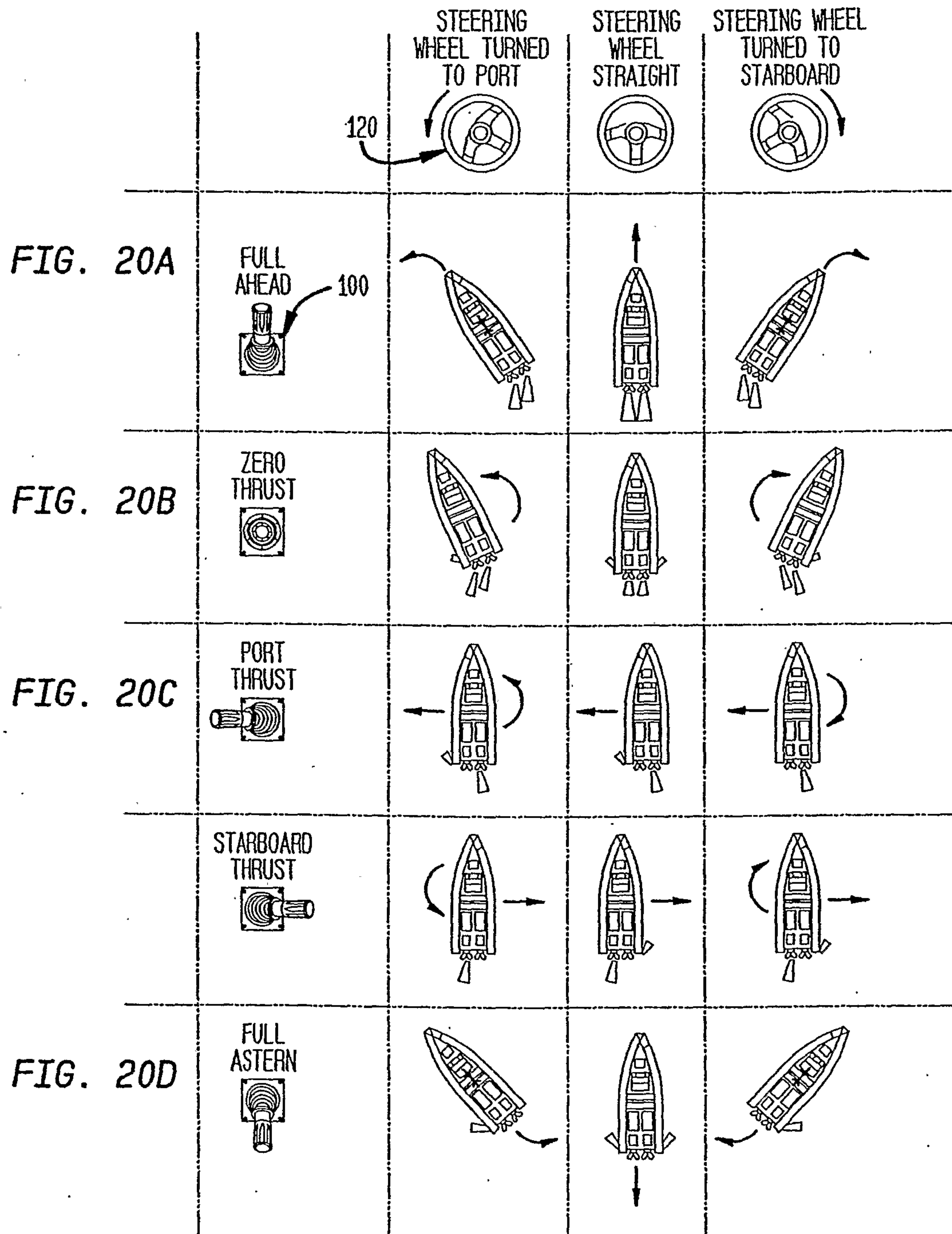
FIG. 20 DUAL WATERJET MOTION DIAGRAM
