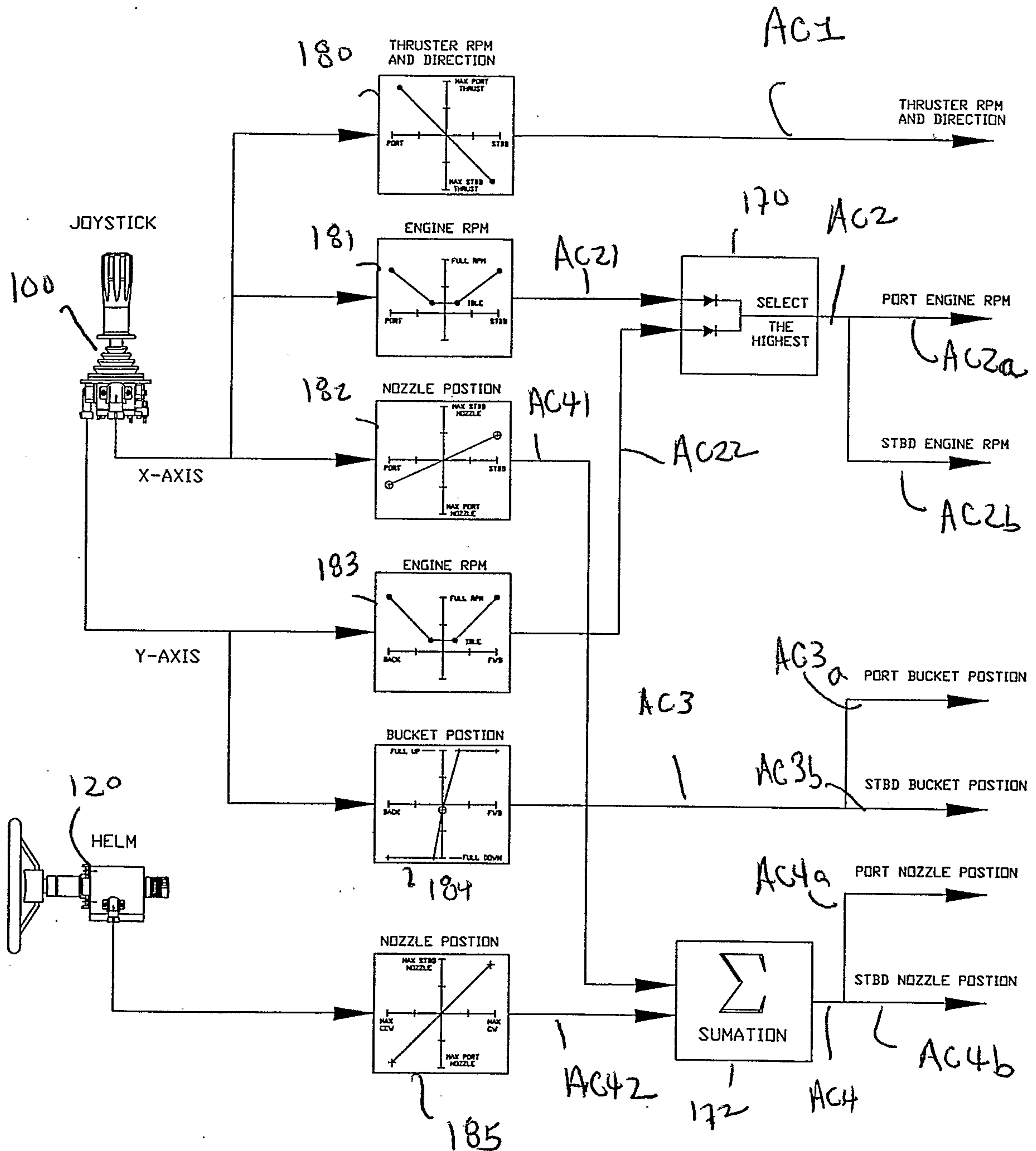
FIG 32 - DUAL WATERJET WITH BOW THRUSTER SIGNAL DIAGRAM
