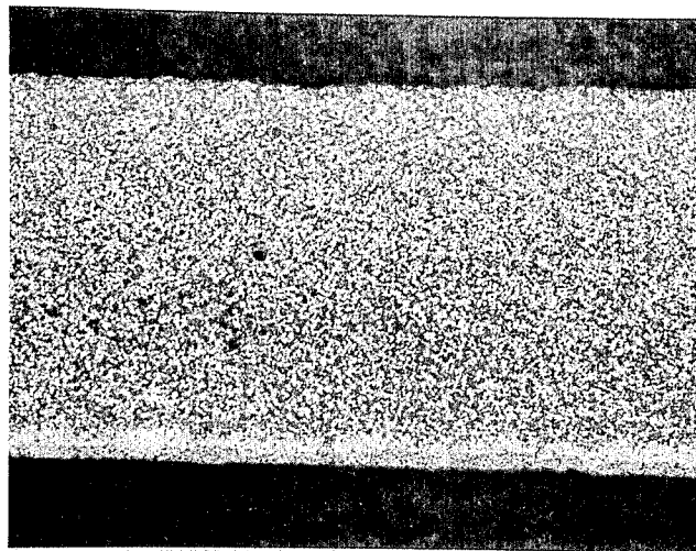
100X Picral Etch 3J960 a. Microstructure of Casting Cross Section
