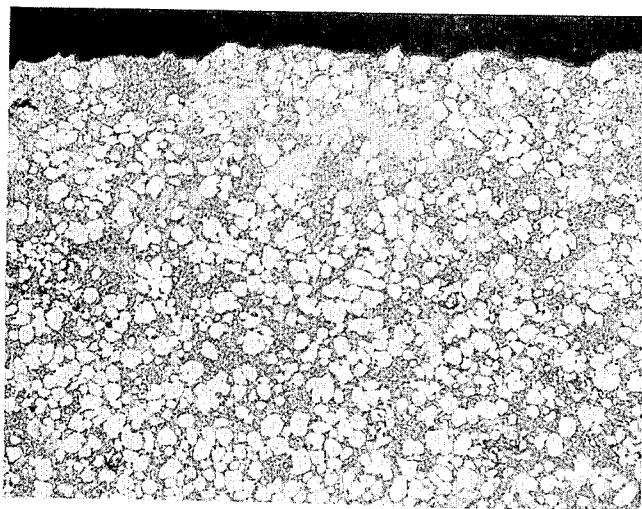
500X Picral Etch 3J961 b. Microstructure Adjacent to the Cover Die Surface
