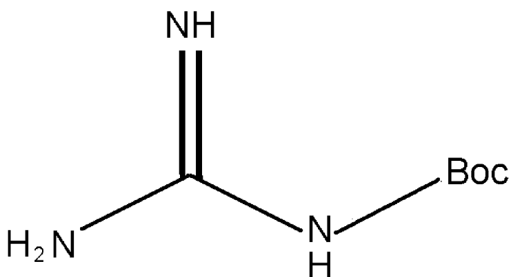
[Chemical Formula 20]
