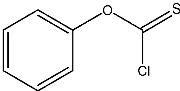
[Chemical Formula 13]
