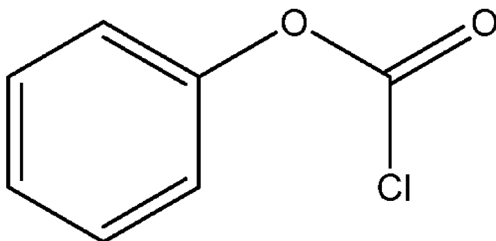
[Chemical Formula 13]
