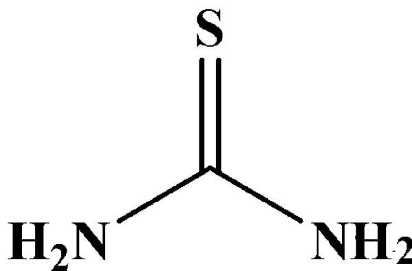
[Chemical Formula 21]
