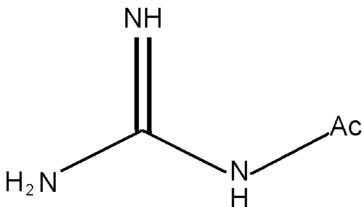
[Chemical Formula 19]
