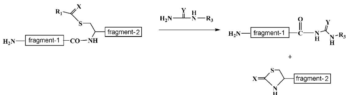
[Chemical Formula 22]
