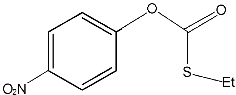
[Chemical Formula 11]
