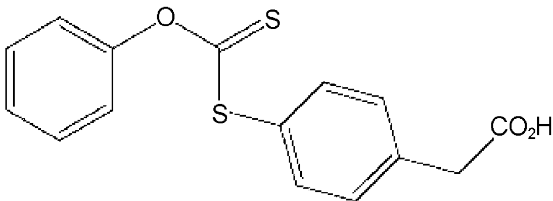
[Chemical Formula 15]
