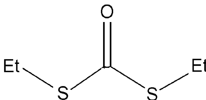
[Chemical Formula 11]
