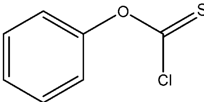
[Chemical Formula 9]
