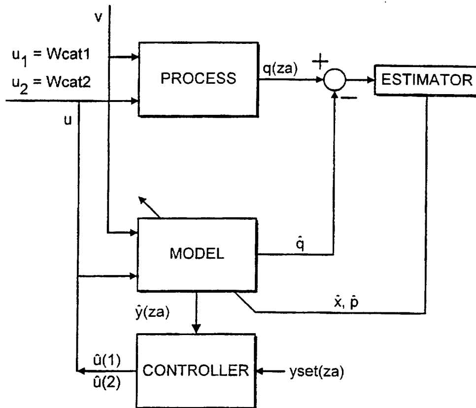
FIG. 2 PROCESS AND MODEL WITH ESTIMATOR AND CONTROLLER
