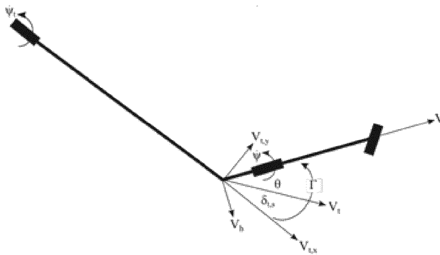
FIGURE 6 VEHICLE/TRAILER MODEL (STATES)
