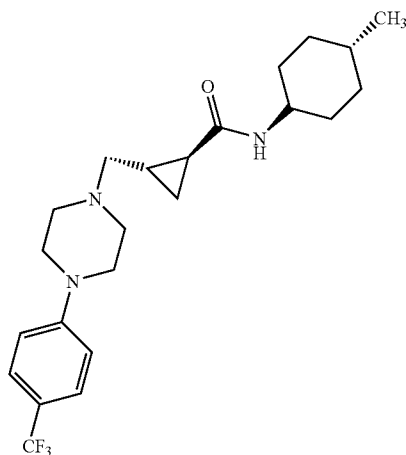
trans-2-[4-(4-Trifluoromethyl-phenyl)-piperazin-1-ylmethyl]cyclopropanecarboxylic acid trans-(4-methylcyclohexyl)-amide
