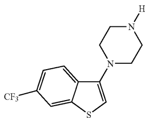
1-(6-(trifluoromethyl)-benzo[b]thien-3-yl)-piperazine hydrochloride
