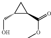
4a: trans-2-Hydroxymethyl-cyclopropanecarboxylic acid methyl ester
