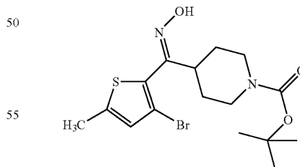
30b: Preparation of 4-[1-(3-bromo-5-methylthiophen-2-yl)-1-hydroxyimino-methyl]-piperidine-1-carboxylic acid tert-butyl ester
