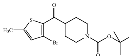
30a: Preparation of 4-[1-(3-bromo-5-methylthiophen-2-yl)-1-methanoyl]-piperidine-1-carboxylic acid tert-butyl ester
