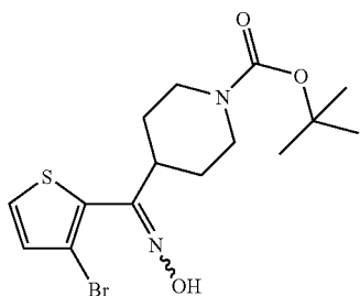
21b: 4-[(3-Bromo-thiophen-2-yl)-hydroxyimino-methyl]-piperidine-1-carboxylic acid tert-butyl ester
