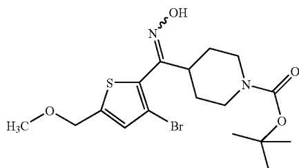
31d: Preparation of 4-[1-(3-bromo-5-methoxymethyl-thiophen-2-yl)-1-hydroxyimino-methyl]-piperidine-1-carboxylic acid tert-butyl ester
