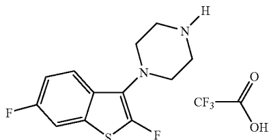
1-(2,6-Difluoro-benzo[b]thien-3-yl)-piperazine trifluoroacetate
