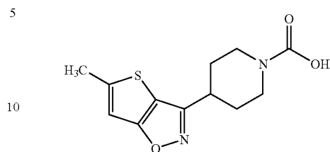
4-(5-Methyl-thieno[2,3-d]isoxazol-3-yl)-piperidine-1-carboxylic acid
