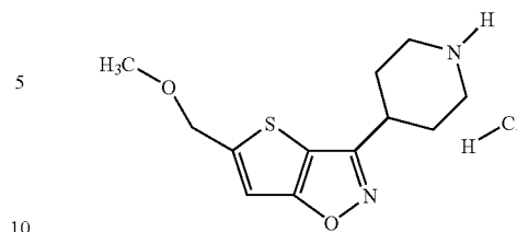
31f: Preparation of 5-methoxymethyl-3-piperidin-4-yl-thieno[2,3-d]isoxazole hydrochloride
