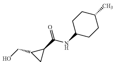
11c: trans-2-Hydroxymethyl-cyclopropanecarboxylic acid trans-(4-methylcyclohexyl)-amide
