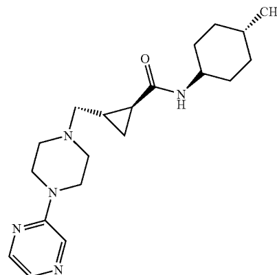
trans-2-[4-(pyrazin-2-yl)-piperazin-1-ylmethyl]-cyclopropanecarboxylic acid trans-(4-methylcyclohexyl)-amide
