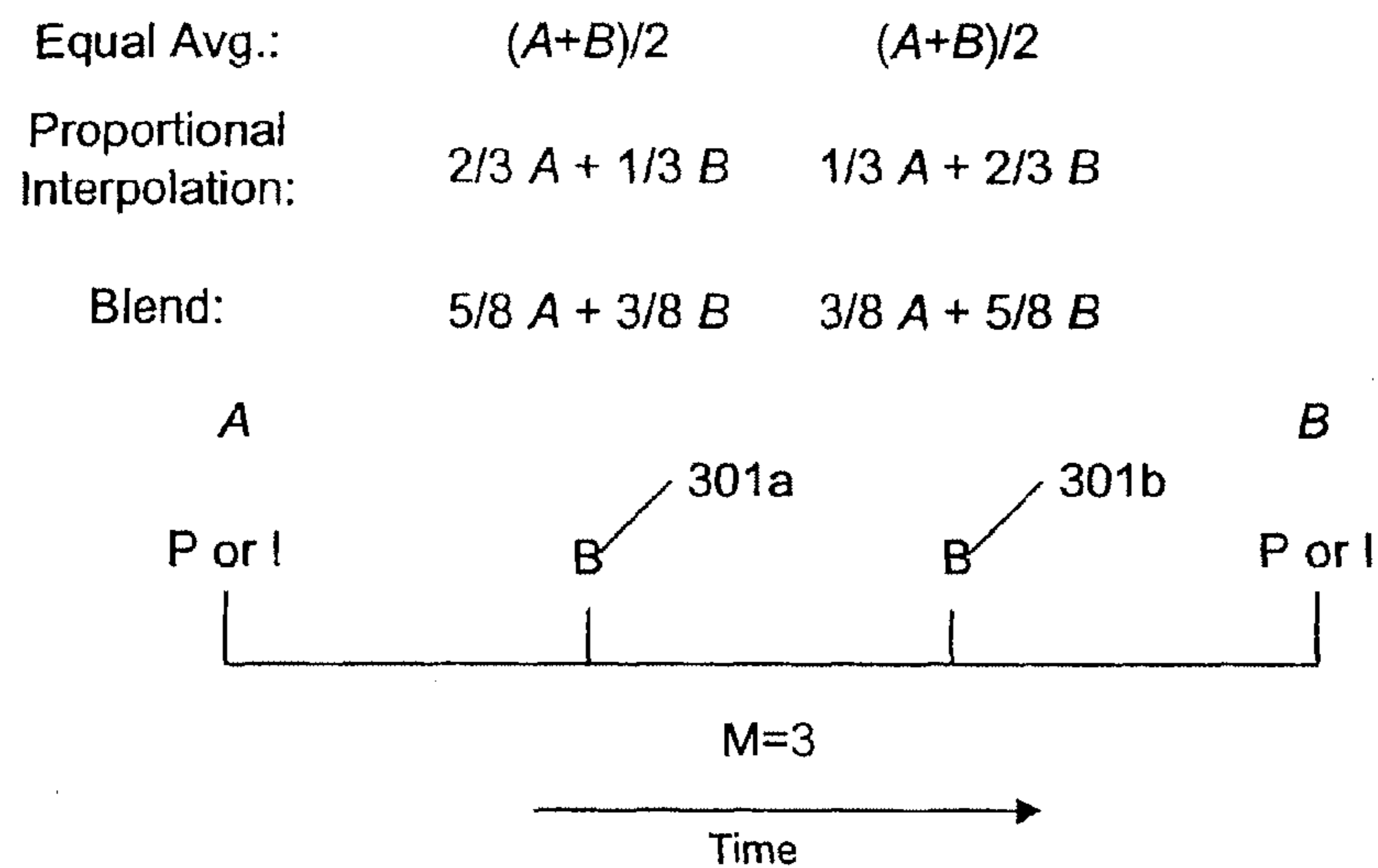
FIG. 3 Blended Pixel Value Weighting
