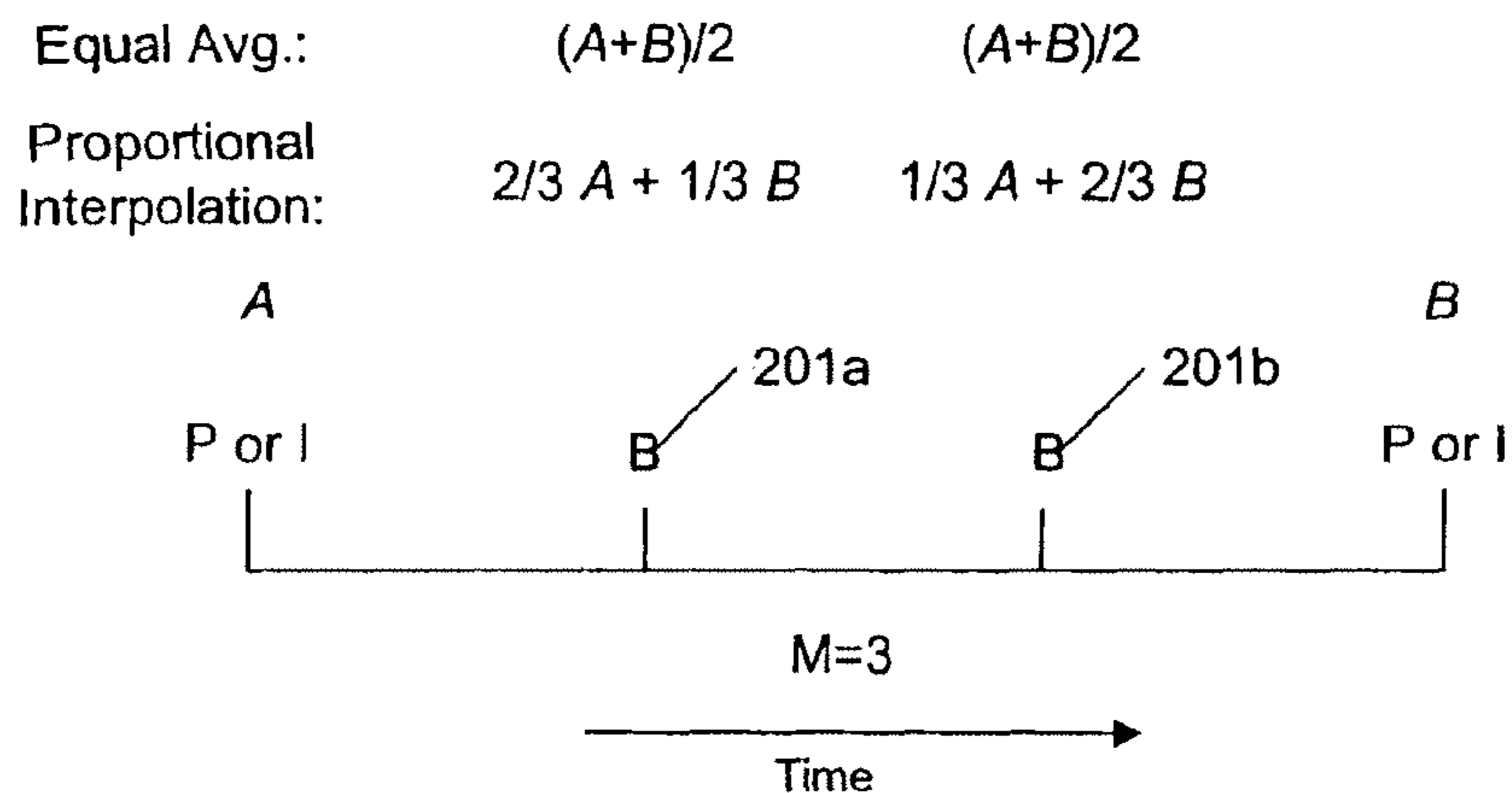
FIG. 2 Pixel Value Proportional Weighting
