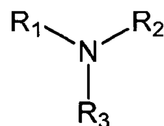
Formula 1
