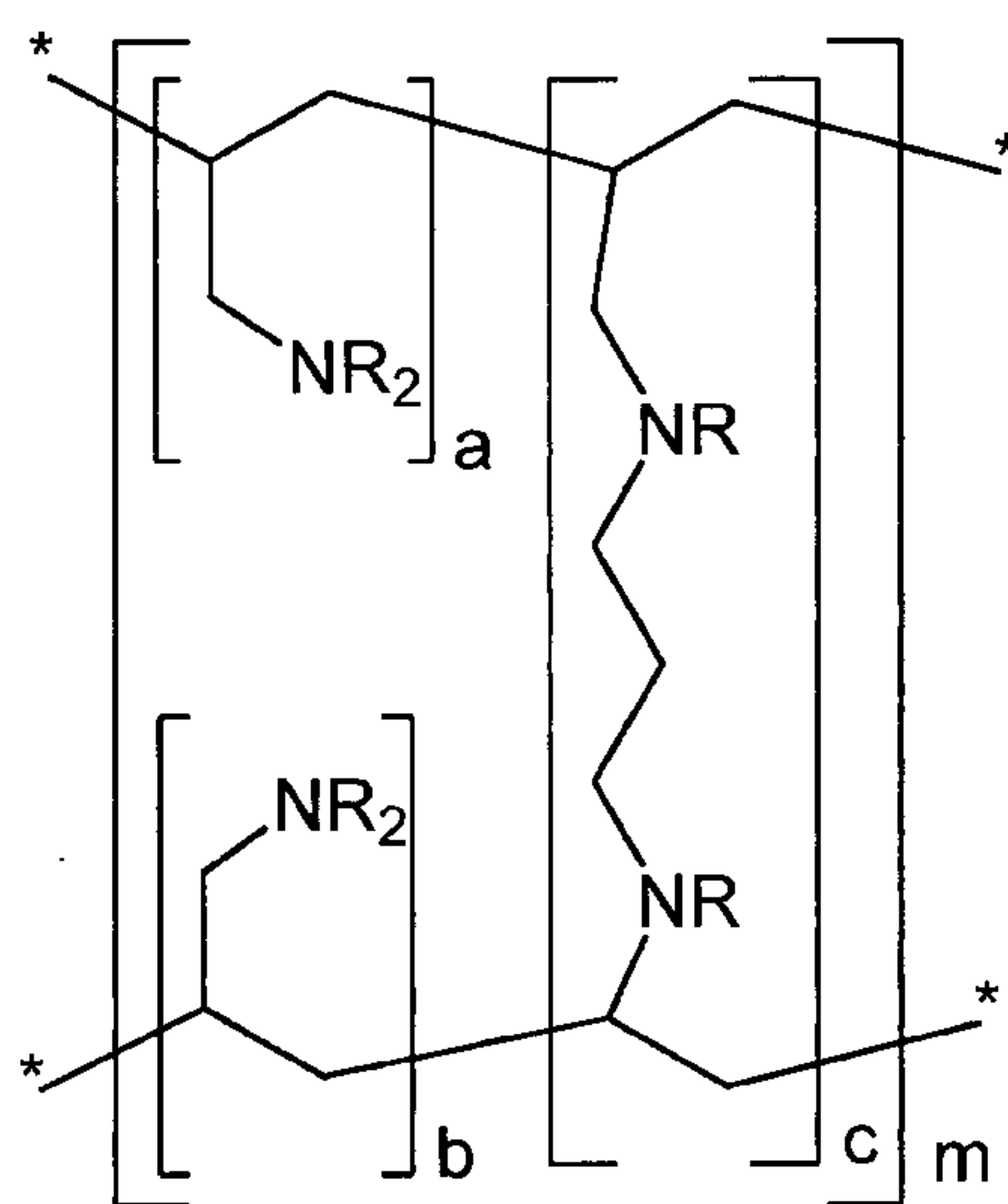
Formula 4
