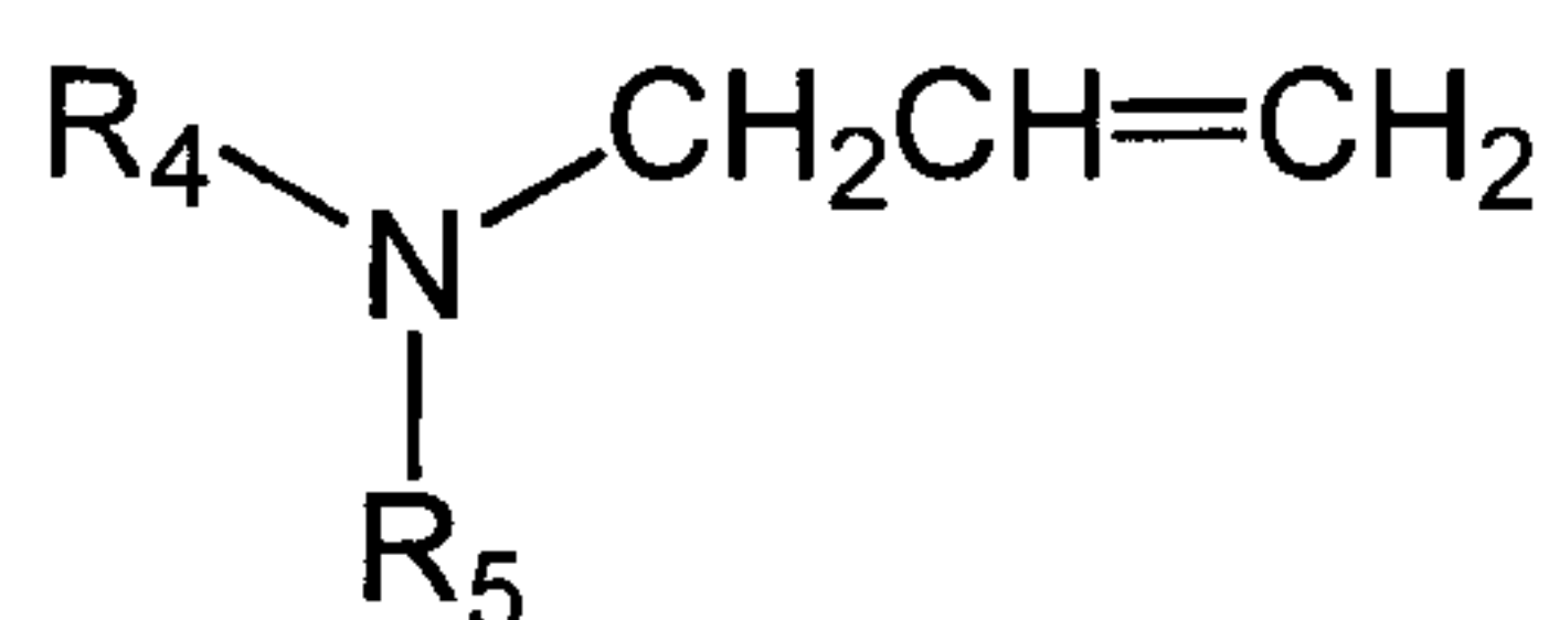
Formula 1a
