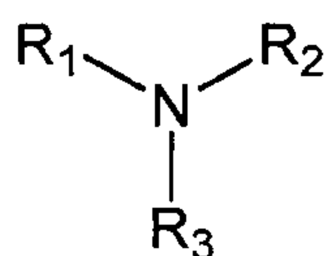
Formula 1
