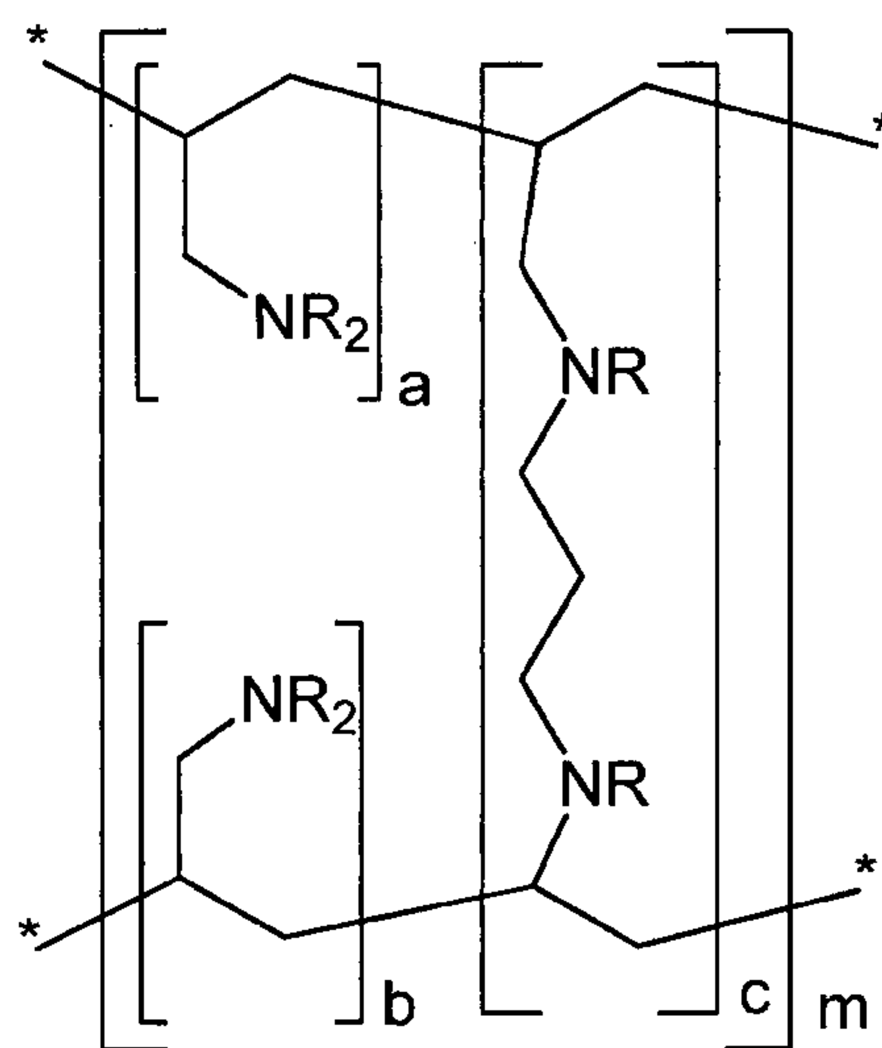
Formula 4
