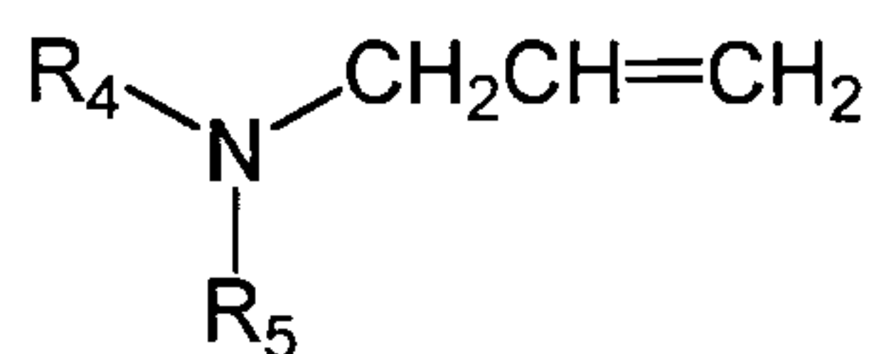
Formula 1a
