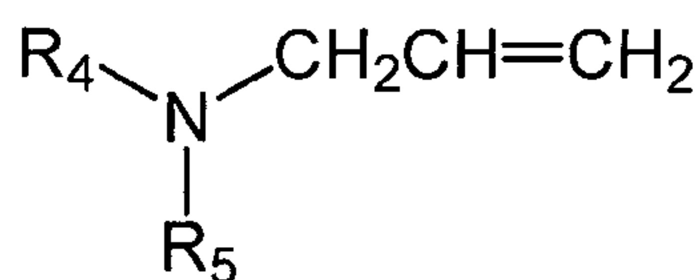
Formula 1a
