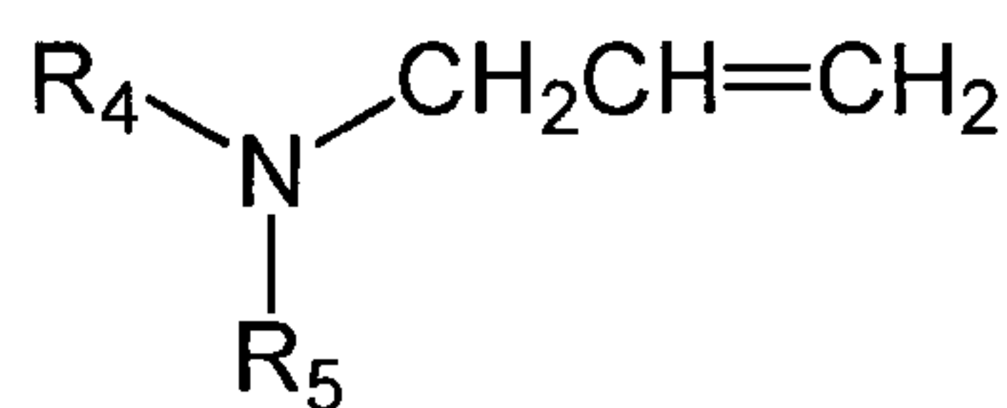
Formula 1a
