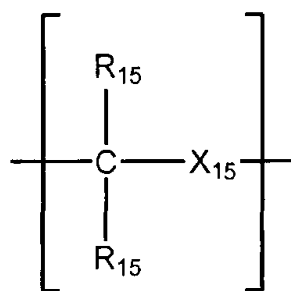
Formula 3
