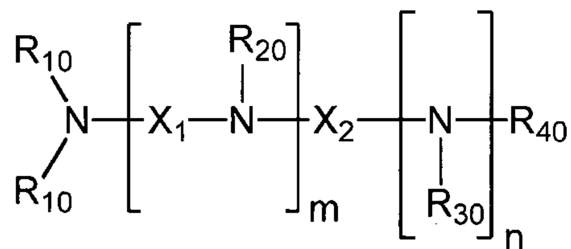
Formula 2
