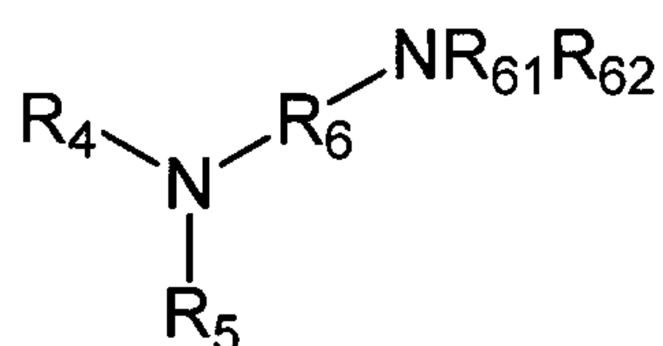
Formula 1b
