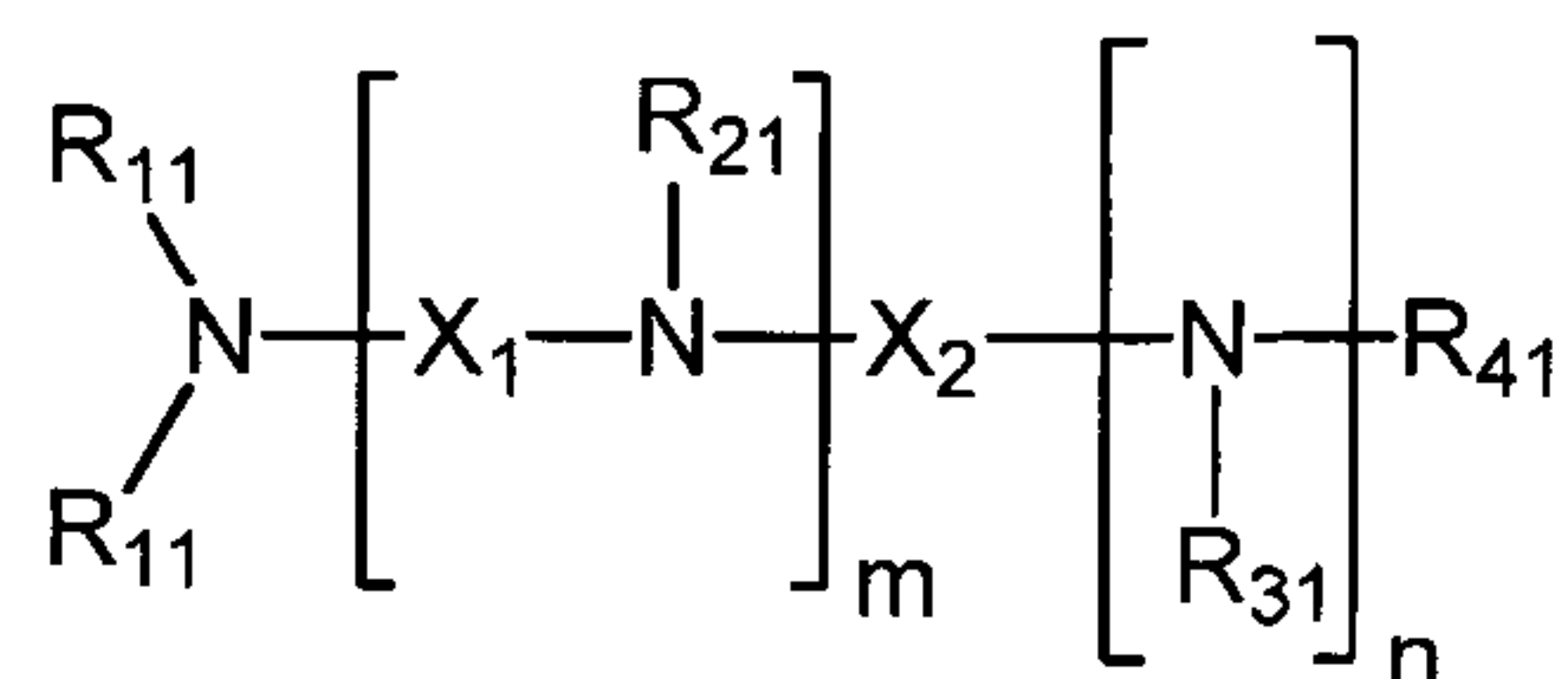
Formula 2a
