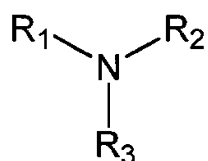
Formula 1
