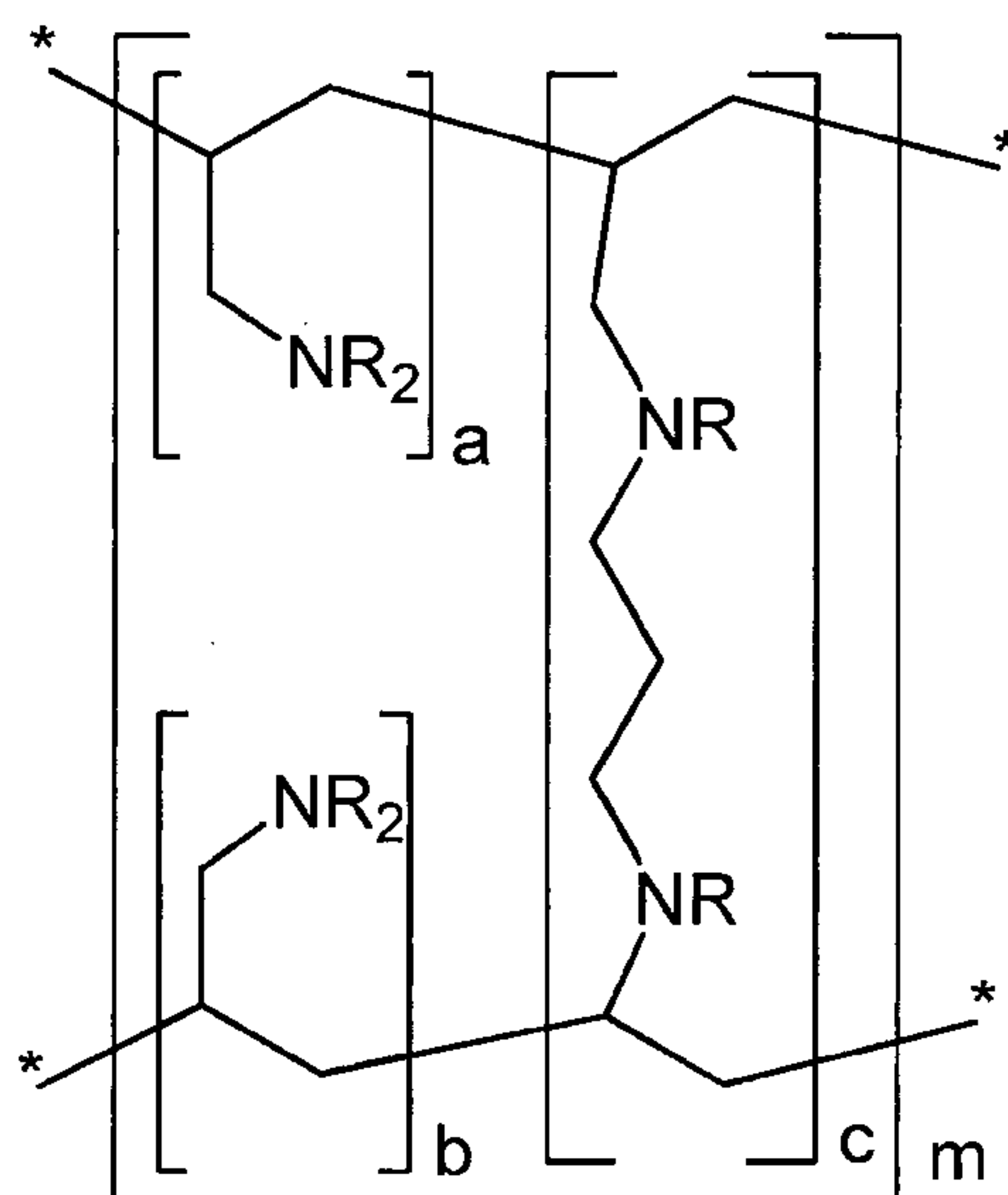
Formula 4
