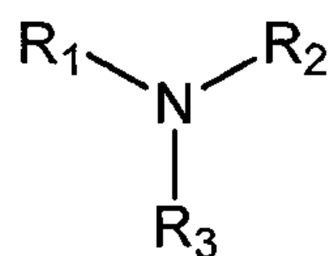
Formula 1
