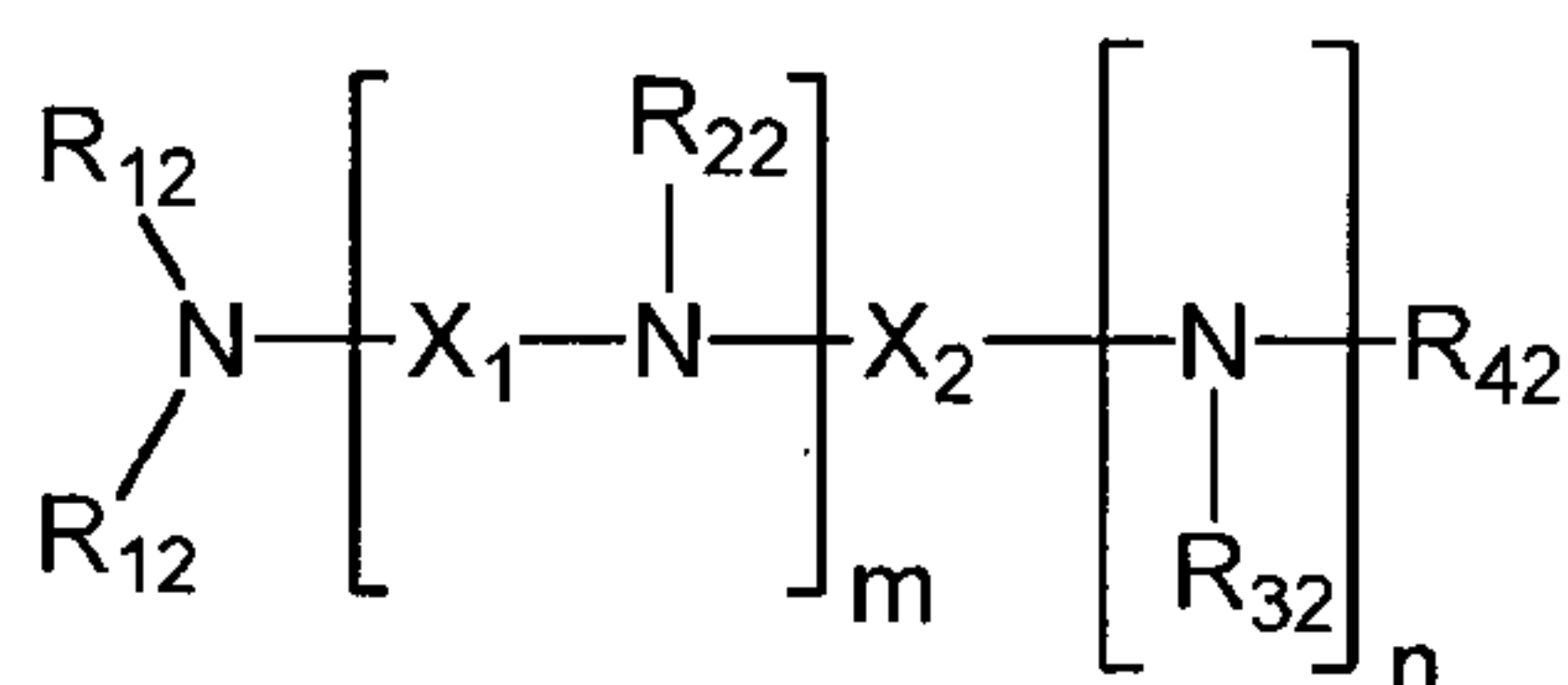
Formula 2b
