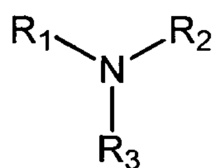
Formula 1
