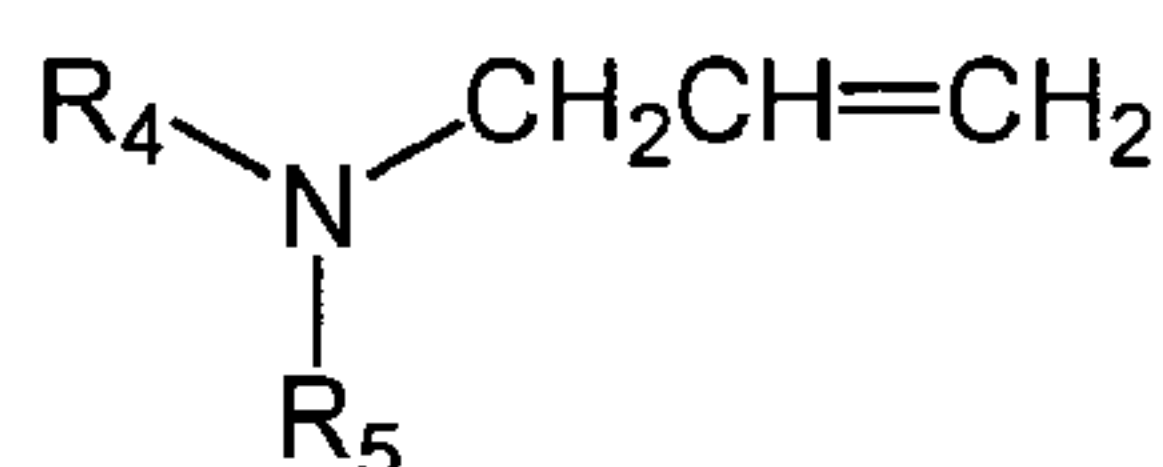
Formula 1a
