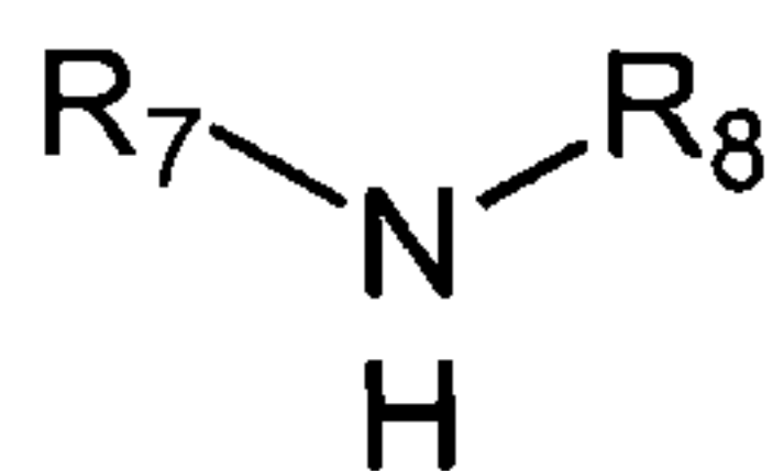
Formula 1c
