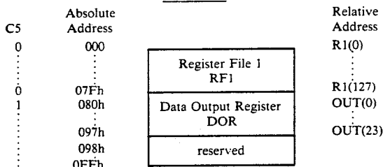
DOR/RF1 Memory Map: h indicates hexadecimal
