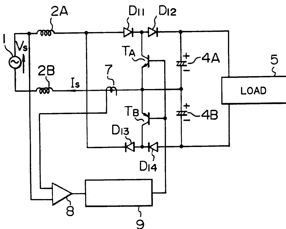
FIG. 16 PRIOR ART
