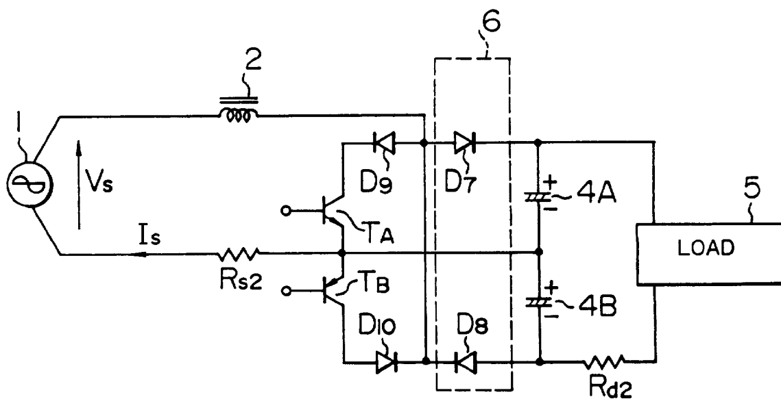
FIG. 15 PRIOR ART
