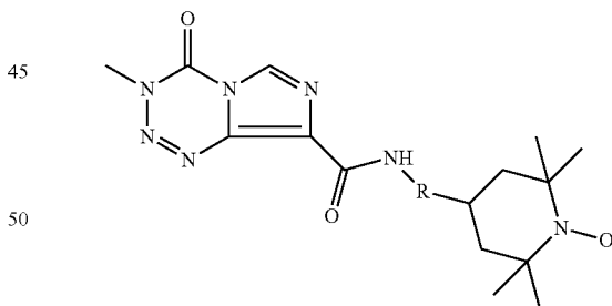
Temozolomide Adduct
