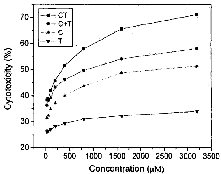
Cytotoxicity of chlorambucil-TEMPOL adduct to KB cells
