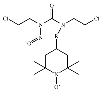
Camustine Adduct
