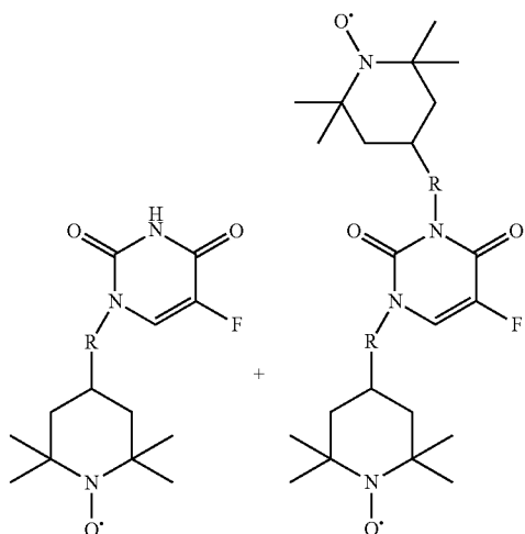
5-fluorouracil Adducts
