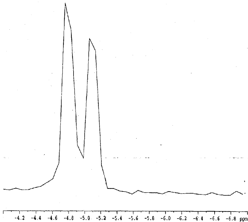
31 P NMR of DNA in the presence of chlorambucil. The change is obvious compared with the 31 P spectrum of the native DNA.
