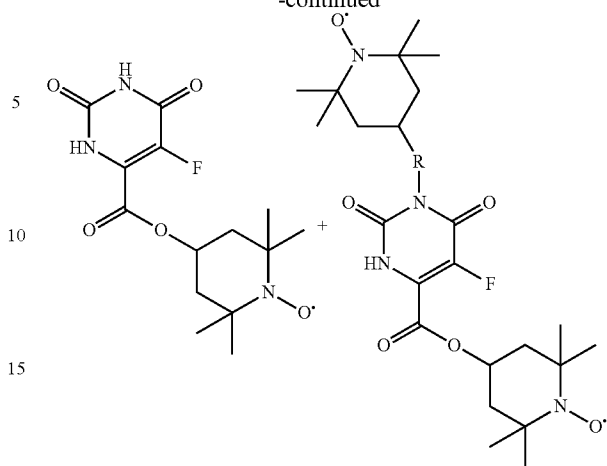
5-fluoroacetic acid Adducts
