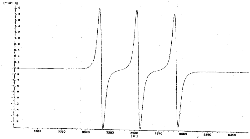
EPR Spectrum of Chromabucil-TEMPOL Adduct
