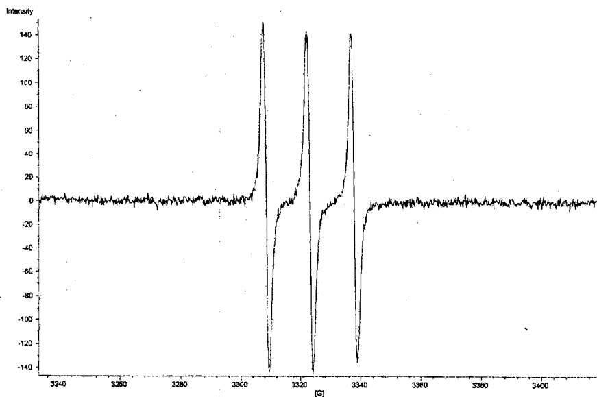
EPR Spectrum of chorambucil-4-Amino-TEMPO Adduct
