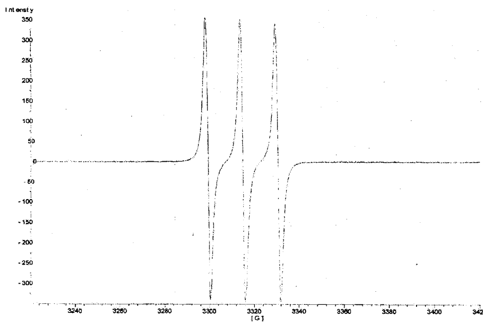
EPR Spectrum of 4-Amino-TEMPO
