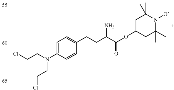
Temozolomide Adduct
