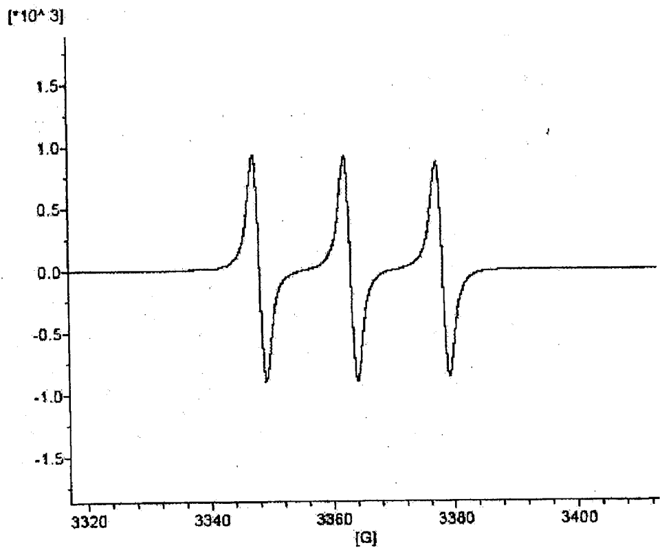
EPR Spectrum of TEMPOL
