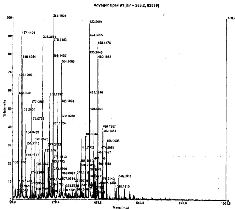
Maldi-TOF Mass Spectrum of chlorambucil-4-Amino-TEMPO
