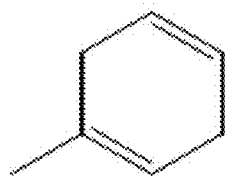
1-methyl-1,4-cyclohexadiene
