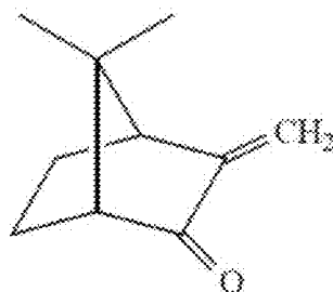
(+)-alpha-methylene-alpha-fenchocamphorone
