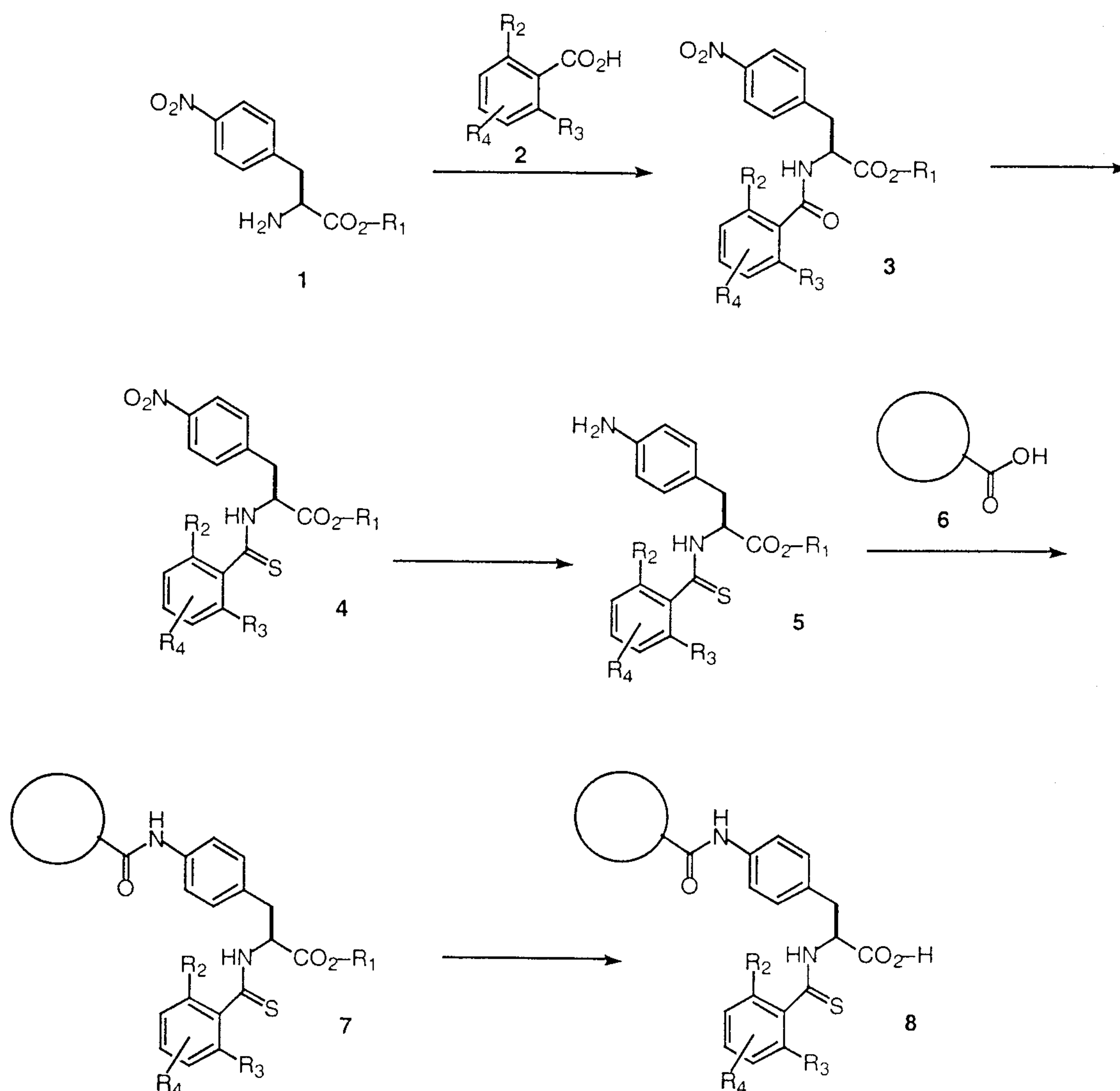
Scheme 1
