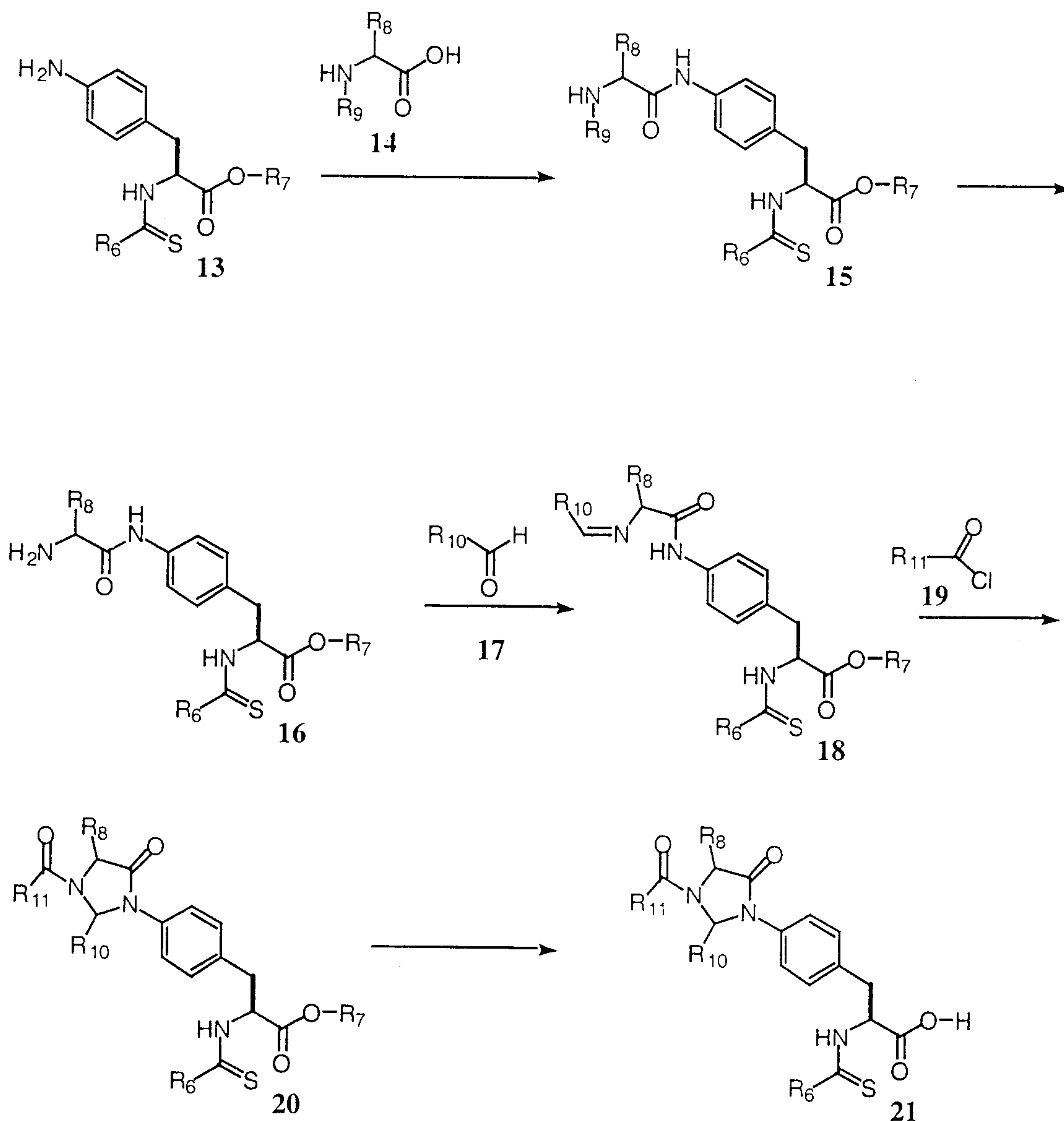
Scheme 3
