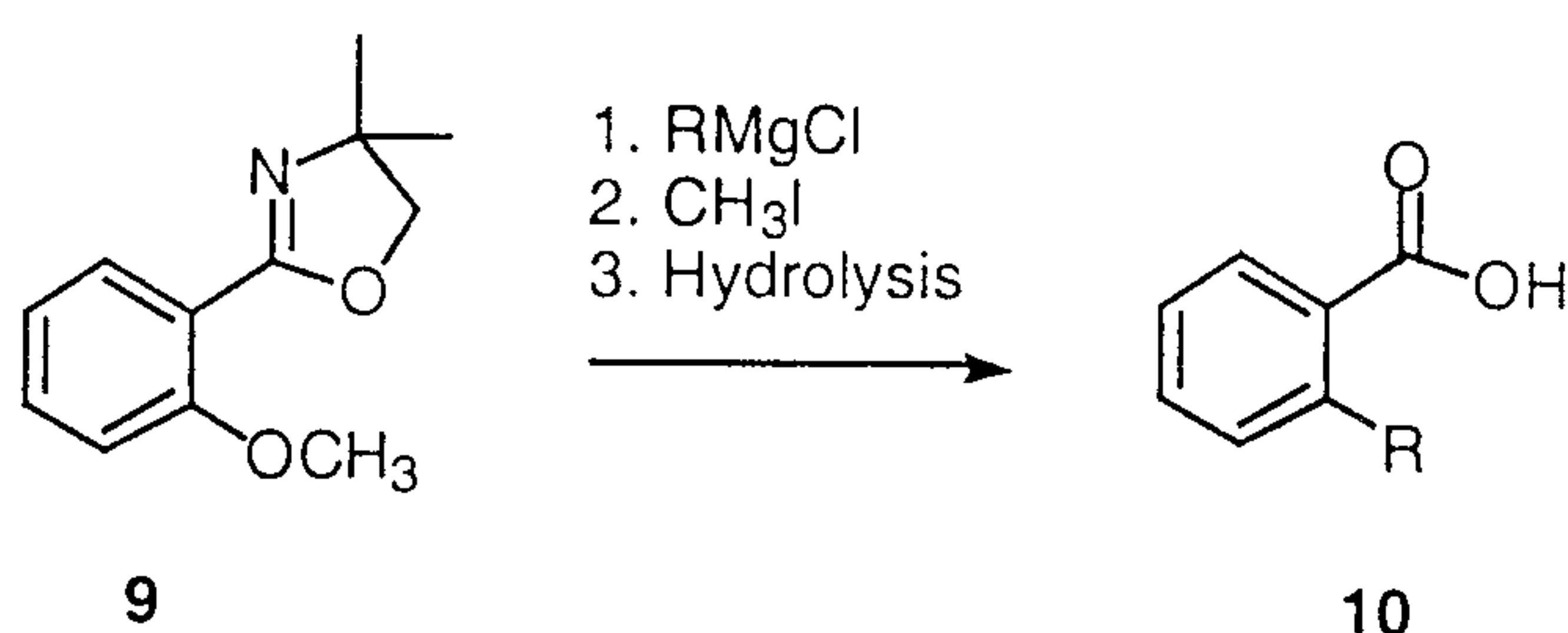
Scheme 2
