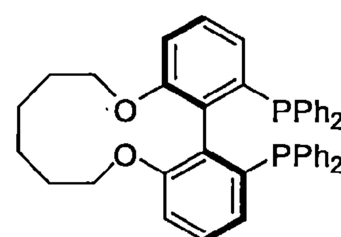
(S)-C6-TunePhos
