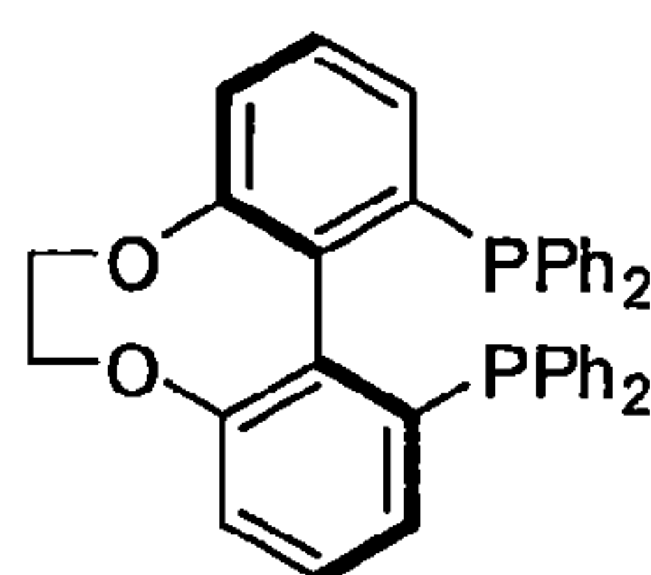
(S)-C2-TunePhos
