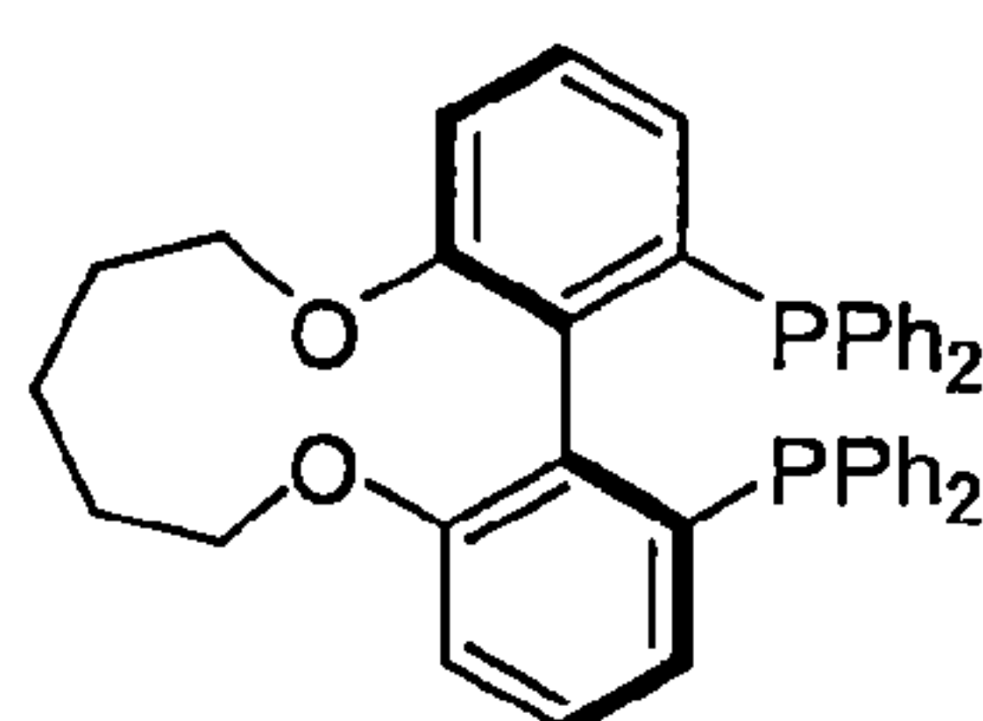
(S)-C5-TunePhos
