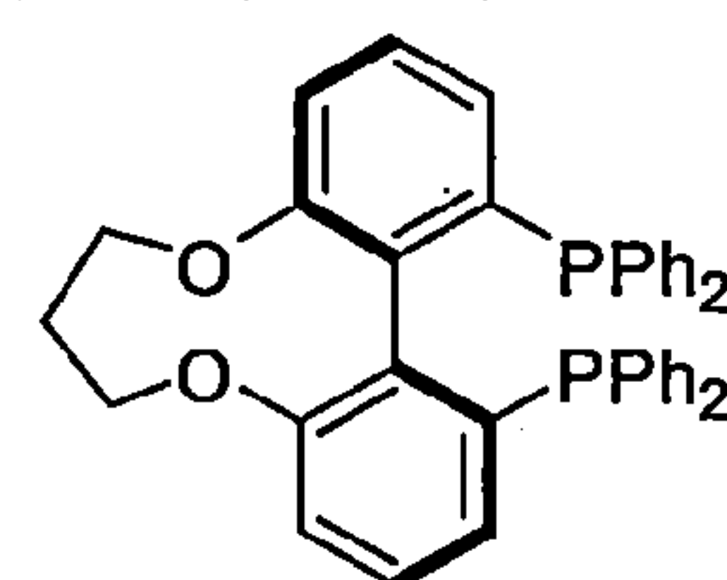
(S)-C3-TunePhos
