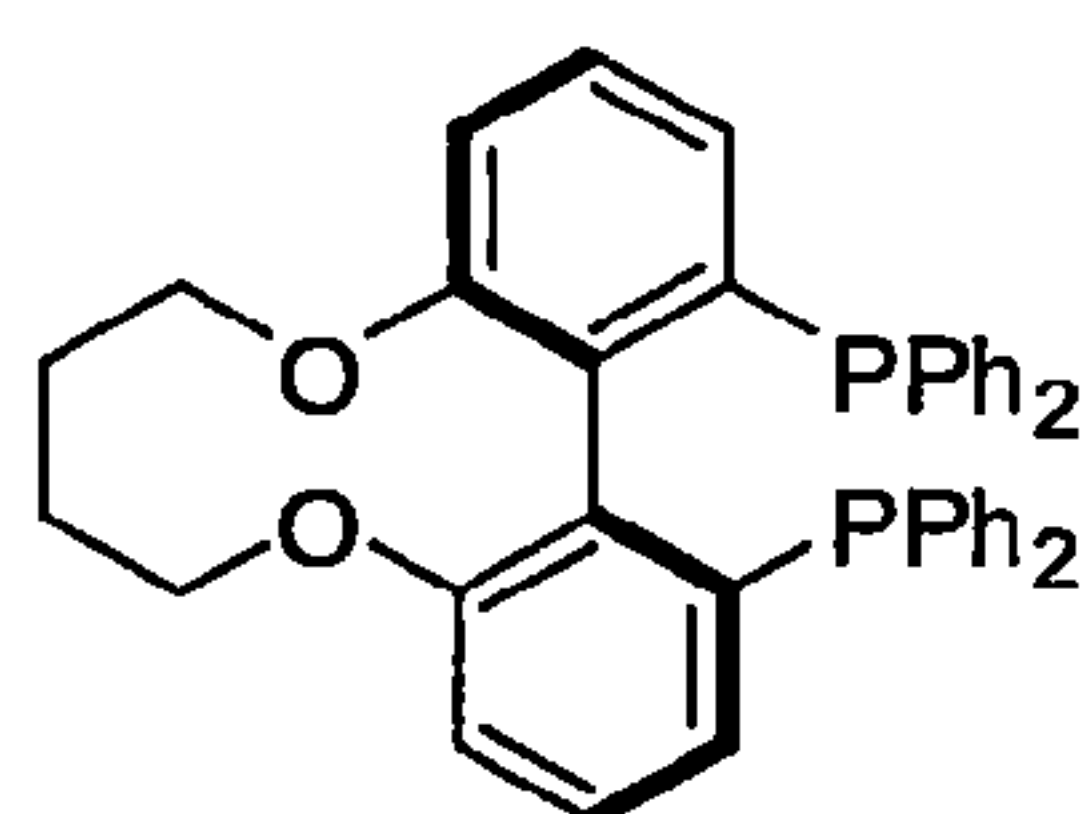
(S)-C4-TunePhos
