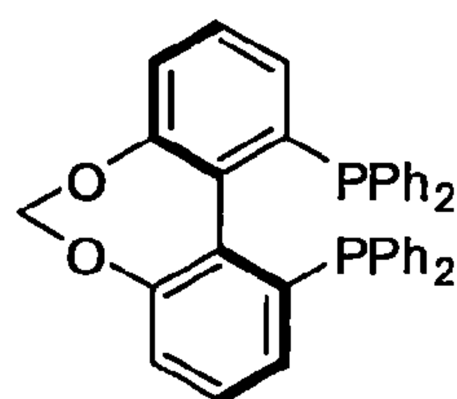
(S)-C1-TunePhos
