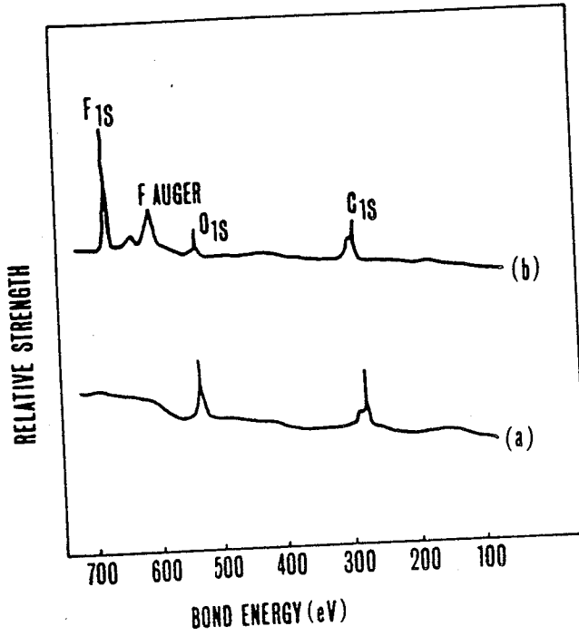
ESCA SPECTRA OF PAINT COATED STEEL SHEET OF EXAMPLE 6 (a) BEFORE PLASMA TREATMENT (b) AFTER PLASMA TREATMENT
