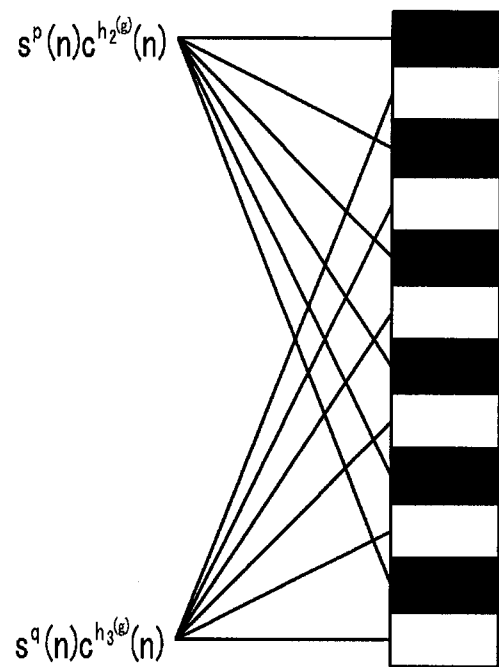
Secondary synchronization signal of sub-frame 5
