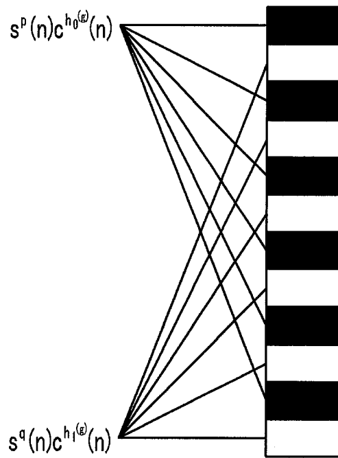
Secondary synchronization signal of sub-frame 0
