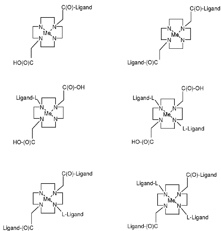
Schematic structures of DO2S derivative-1 conjugates
