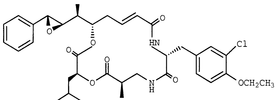
B-7
