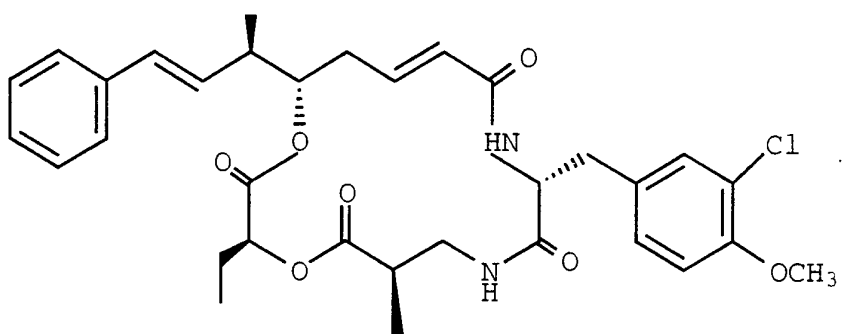
Cryptophycin-214
