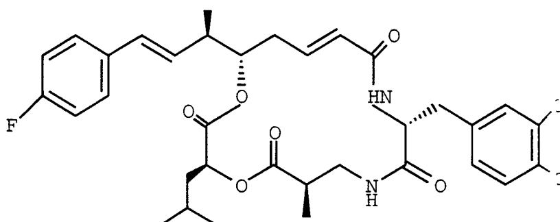
CRYPTOPHYCIN-115
