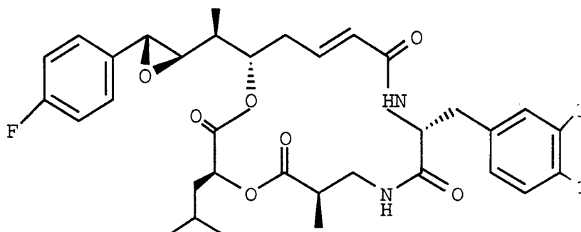
CRYPTOPHYCIN-115
