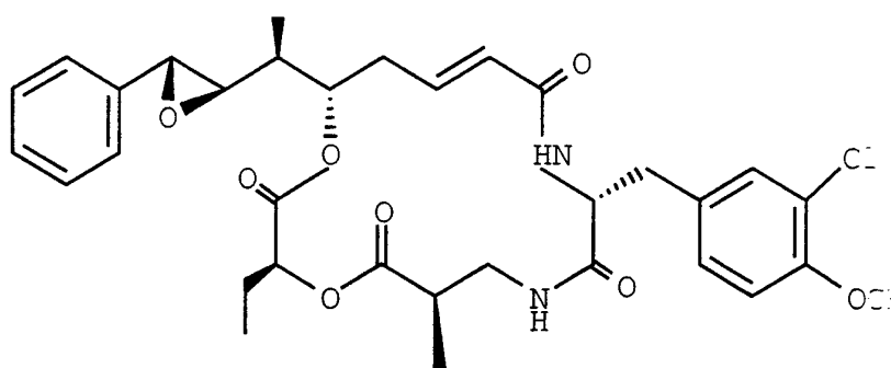
CRYPTOPHYCIN-110
