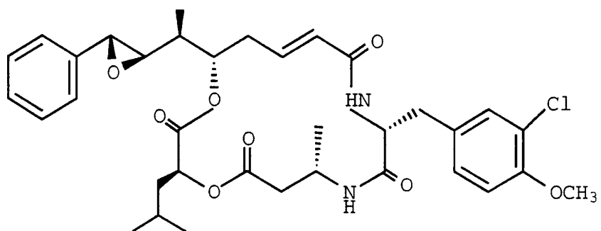
Cryptophycin-213
