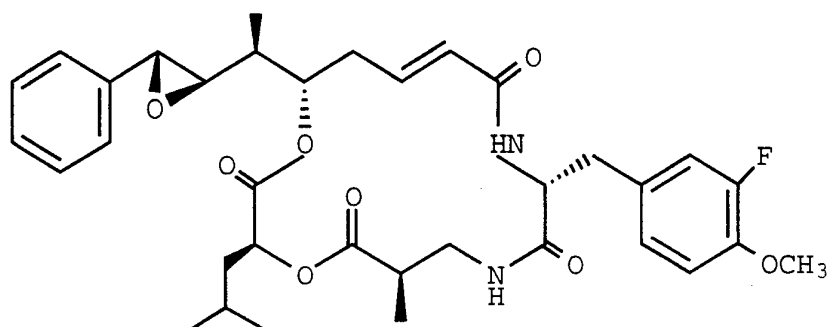
CRYPTOPHYCIN-190
