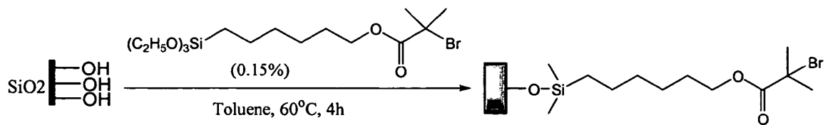
Figure 1: Initiator Molecule Self-assembled into a Monolayer on a Surface.
