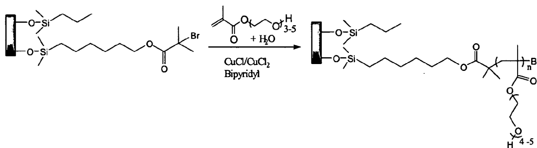
Figure 4: Bonding of PEGAA Polymer Chains to the Initiator Molecules Contained in a SAM Comprised of Both Initiator and Spacer Molecules.
