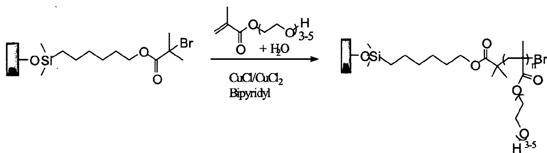
Figure 2: Growing PEGAA Films on a Substrate Using Surface Atom Transfer Radical Polymerization.
