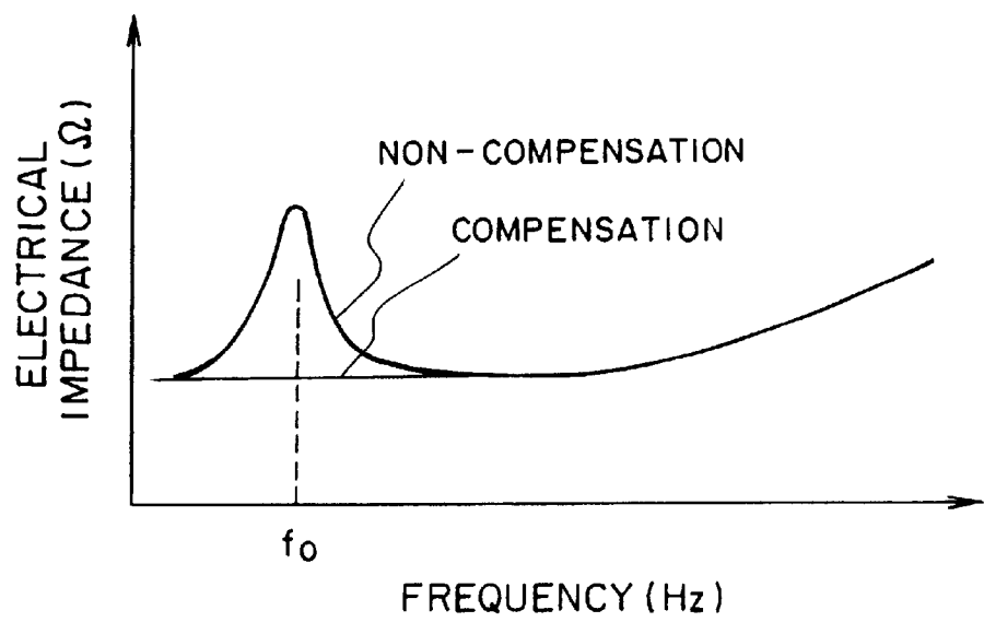
FIG. 8 (PRIOR ART)
