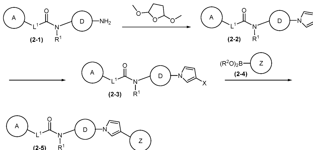
Scheme 2: Representative scheme for synthesis of exemplary compounds of the invention.
