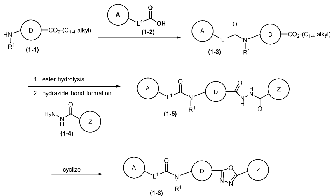
Scheme 1: Representative scheme for synthesis of exemplary compounds of the invention.
