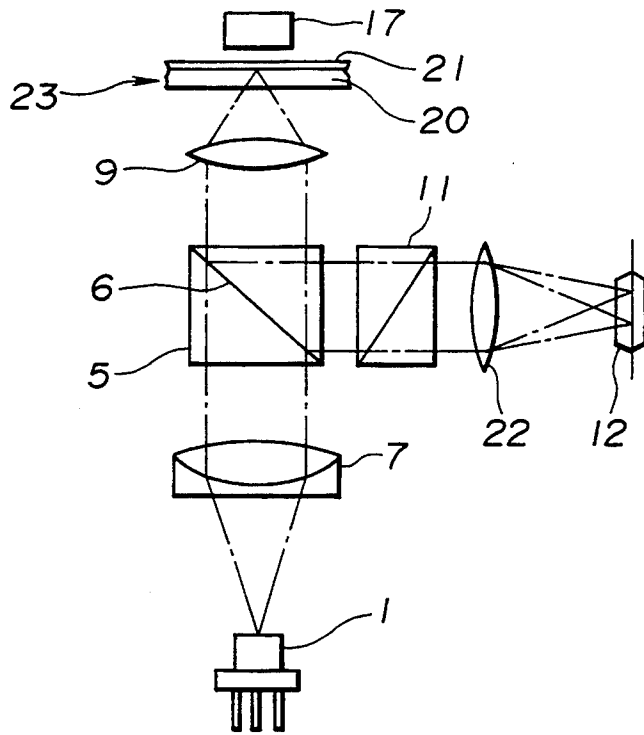
FIG. 1 (PRIOR ART)
