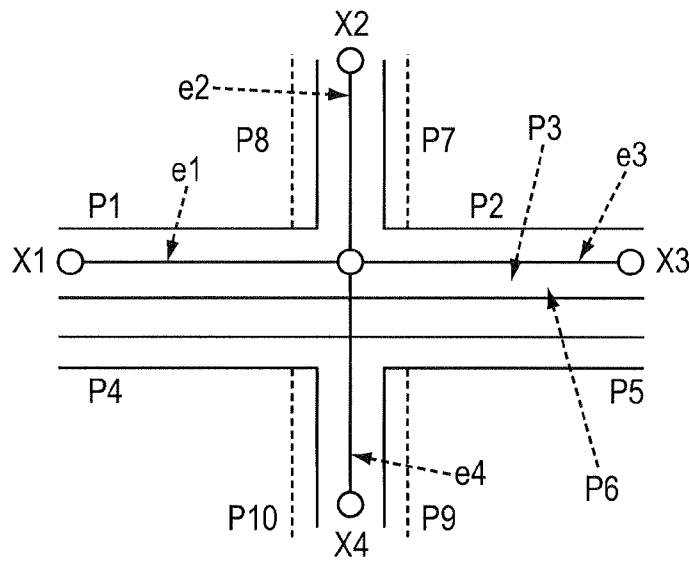
(A) A STAR NETWORK WITH 4 SPOKE NODES
