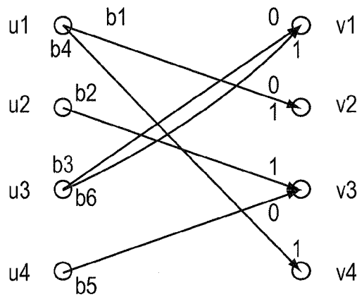
(C) THE BIPARTITE GRAPH G
