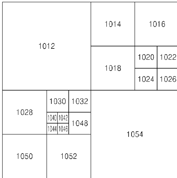
CODING UNITS (1010)
