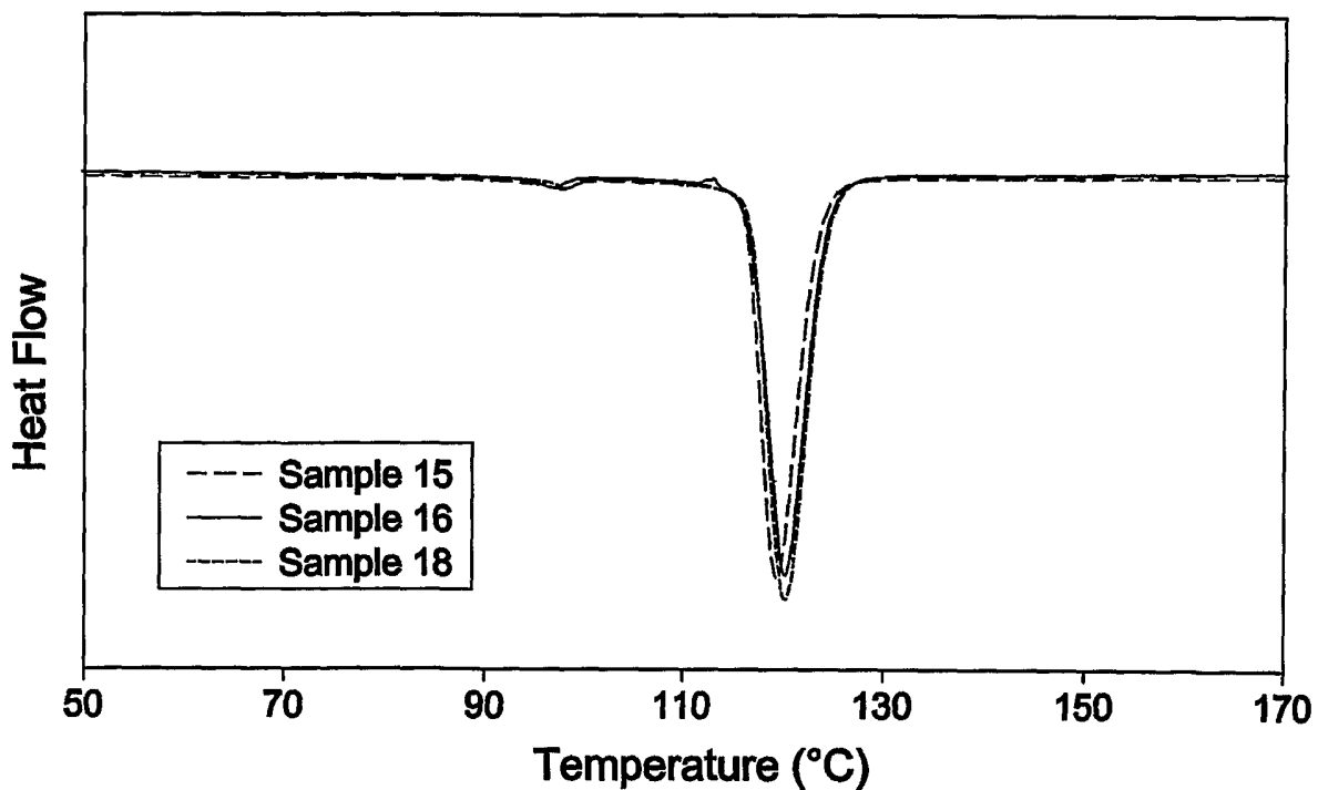
Fig. 10 DSC Crystallization of Plasticized Propylene Impact Copolymers
