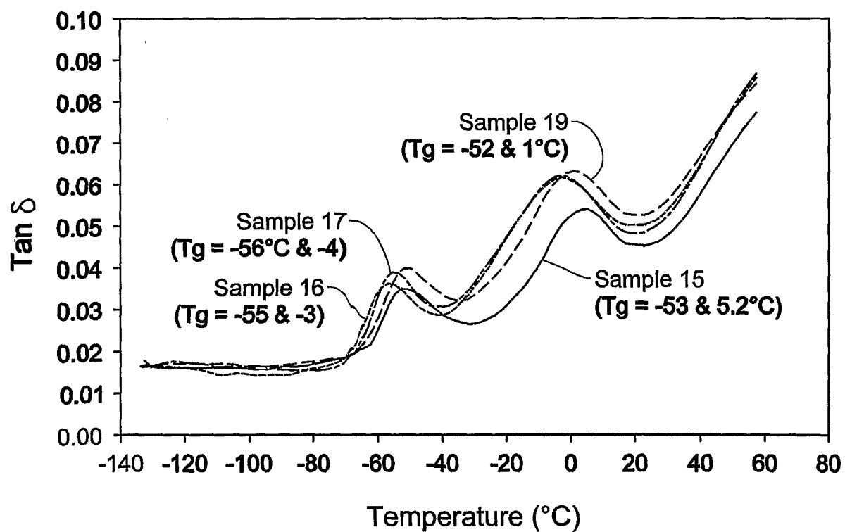
Fig. 4 Tan \delta of Plasticized Propylene Impact Copolymers
