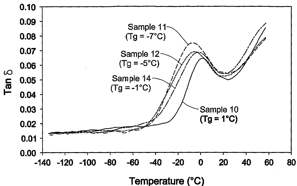
Fig. 3 Tan \delta of Plasticized Propylene Copolymers
