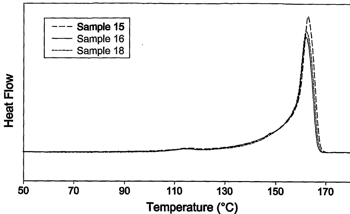
Fig. 9 DSC Melting of Plasticized Propylene Impact Copolymers
