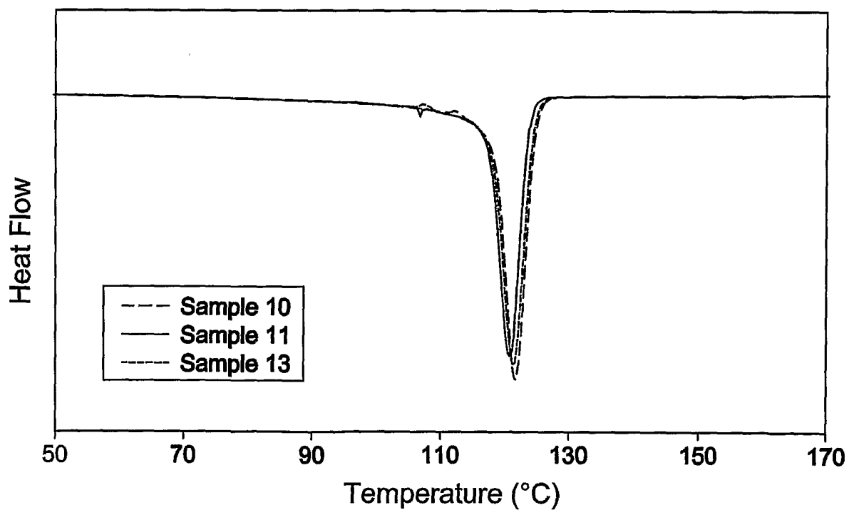
Fig. 8 DSC Crystallization of Plasticized Propylene Random Copolymers
