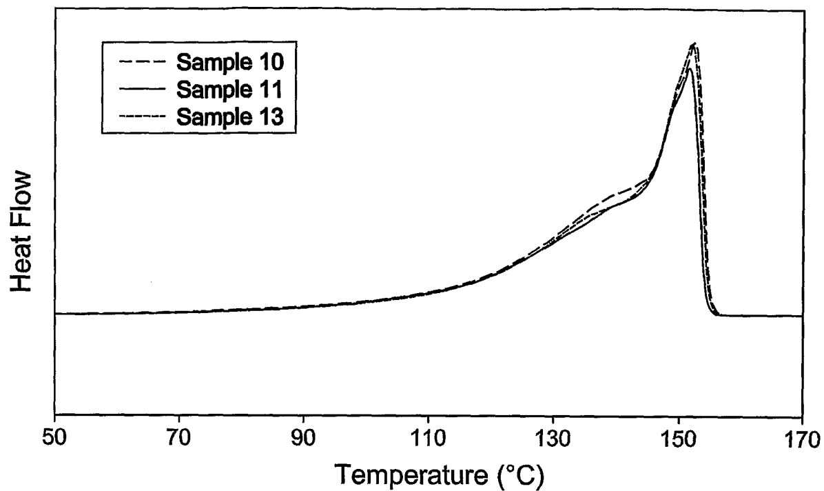
Fig. 7 DSC Melting of Plasticized Propylene Random Copolymers
