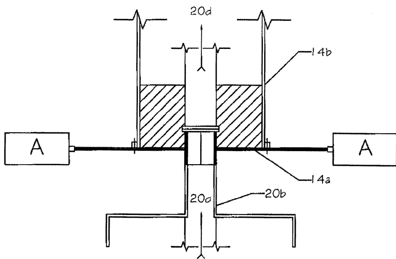
FIGURE 4- SECTION (CLOSED)
