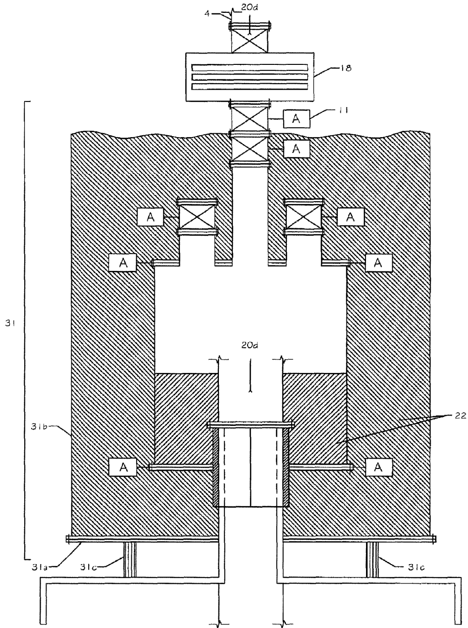
FIGURE 6-PRODUCTION SOLUTION
