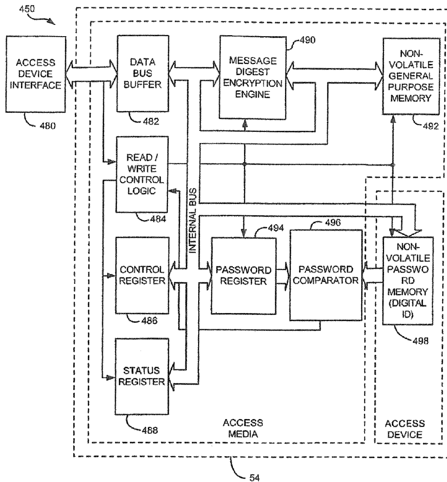
FIG. 21 - HARDWARE TOKEN ACCESS DEVICE
