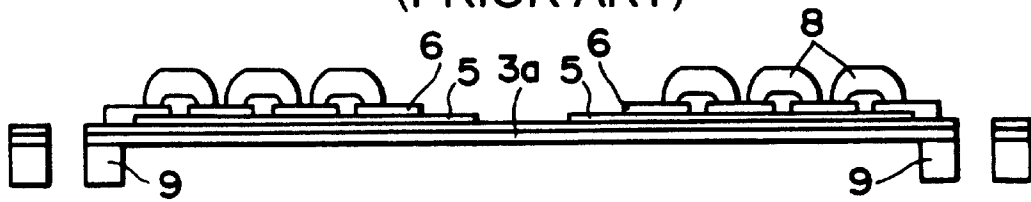
FIG. 11A (PRIOR ART)
