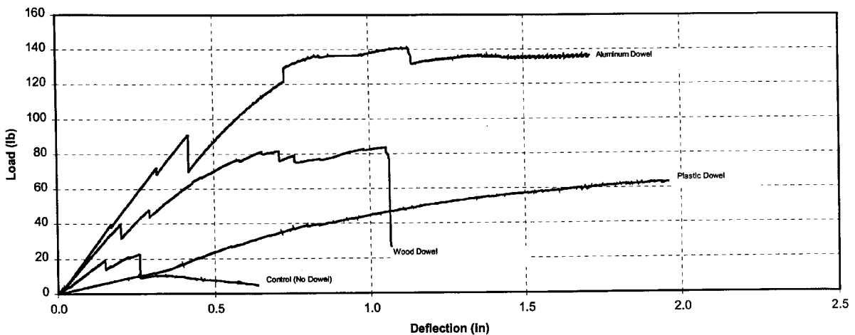
Flexural Properties of Dowel-Reinforced Edge-Glued Panels Bonded with PRF Load vs. Deformation
