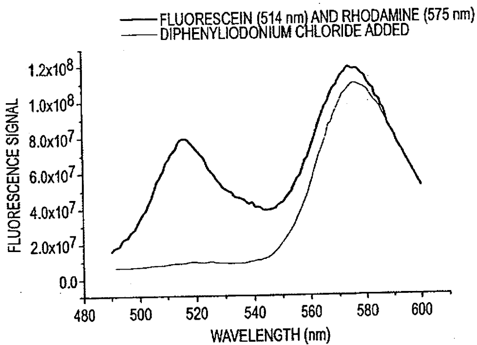
FLUORESCENCE SPECTRA OF EQUIMOLAR FLUORESCHEIN AND TETRA METHYL RHODAMINE BEFORE AND AFTER ADDITION OF DIPHENYLIODONIUM CHLORIDE
