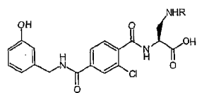
Compound 1, R = (C=S)NH-Fluorescein
