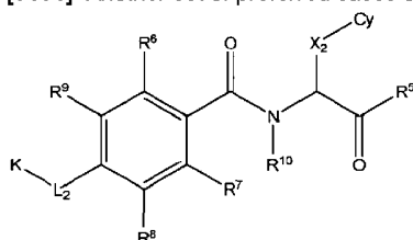
Formula III
