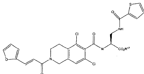
Formula IIA
