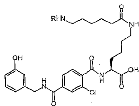
Compound 2A, R = H
