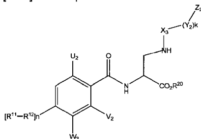
Formula IV
