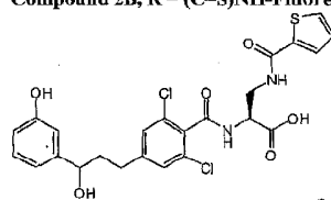
Compound 4
