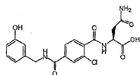
Compound 3
