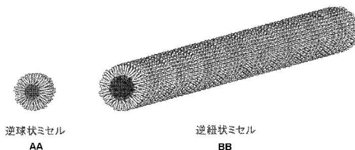
AA REVERSE SPHERICAL MICELLE BB REVERSE THREAD-LIKE MICELLE
