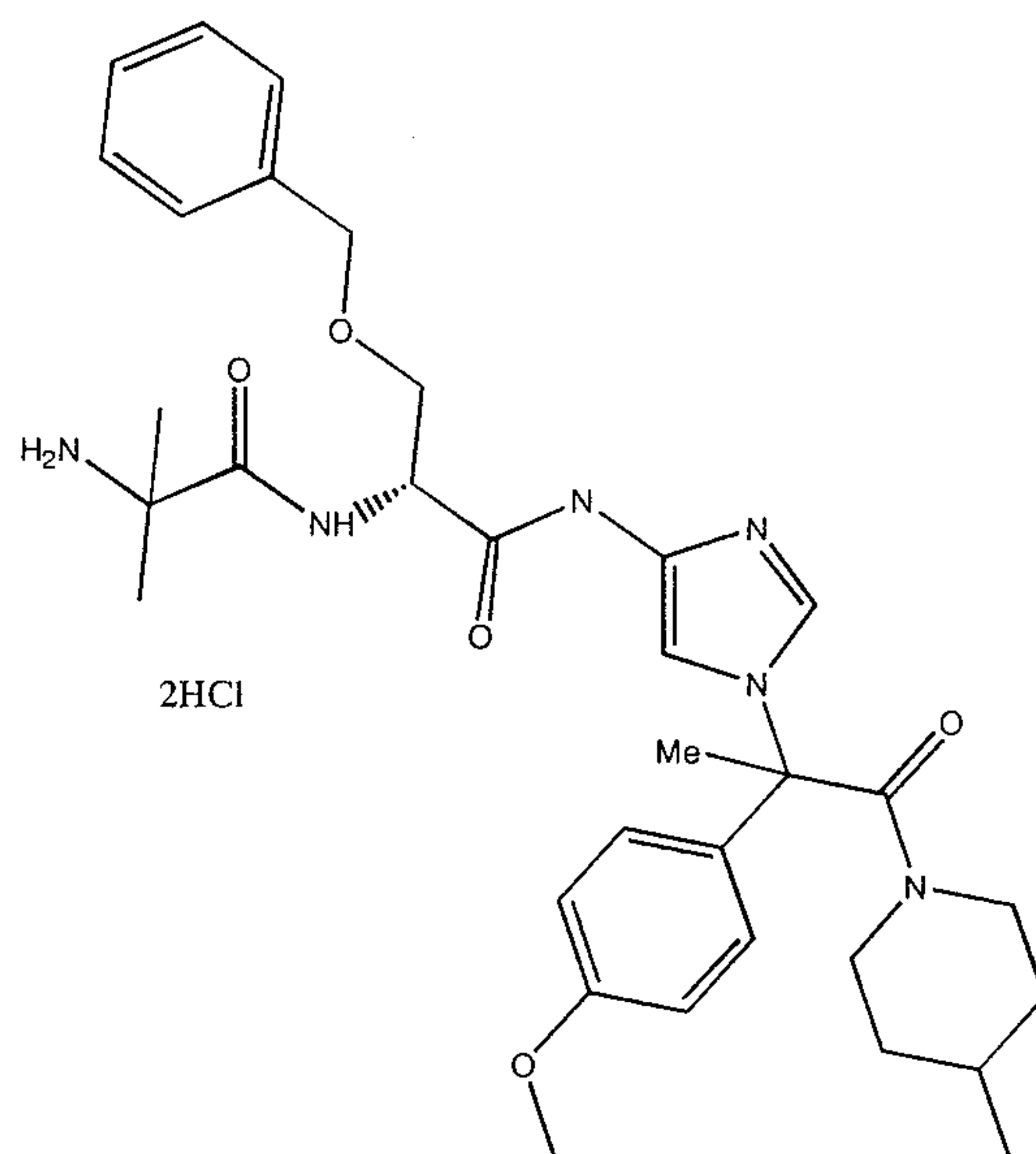
Compound 8
