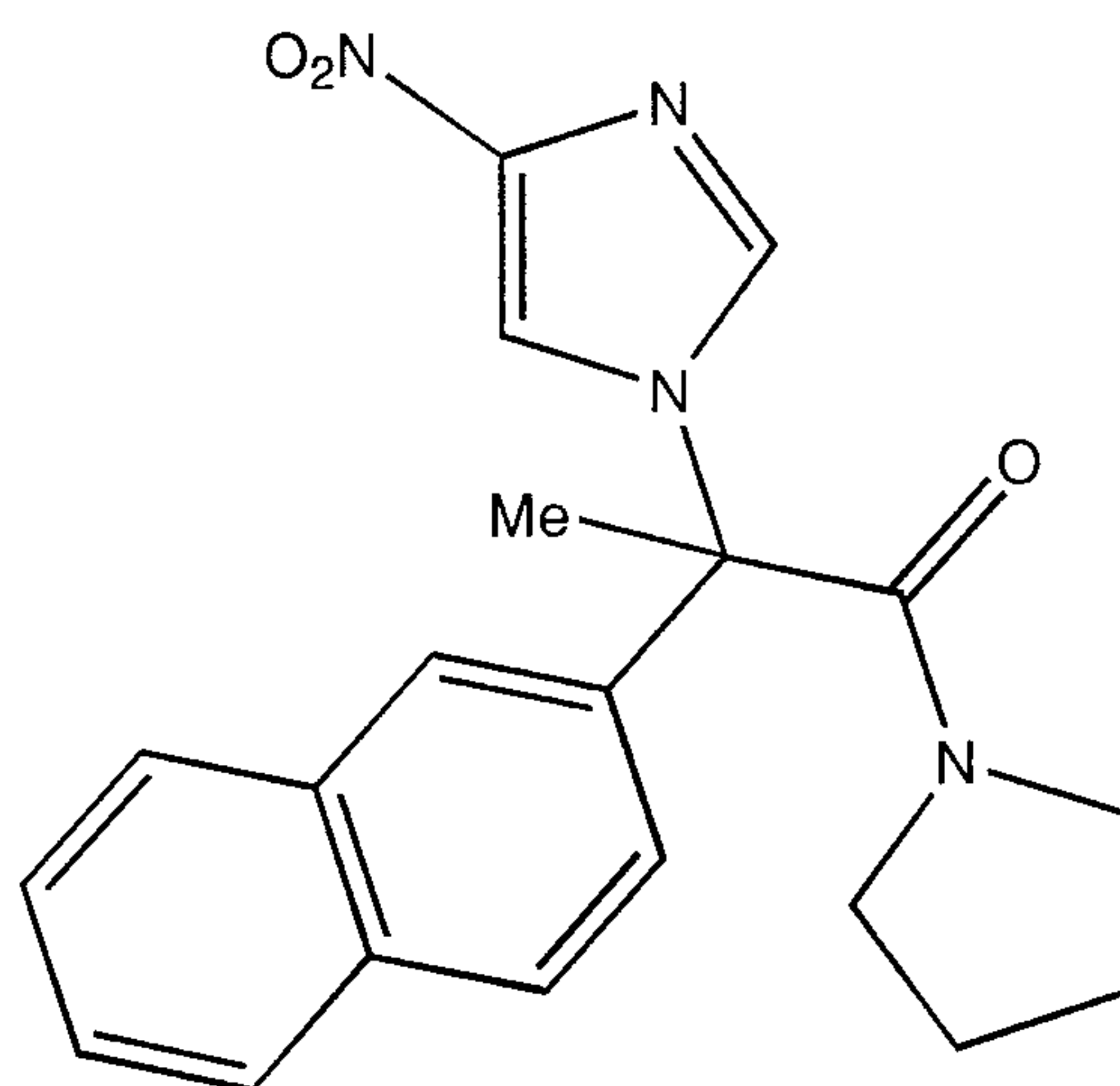
isomer 1
