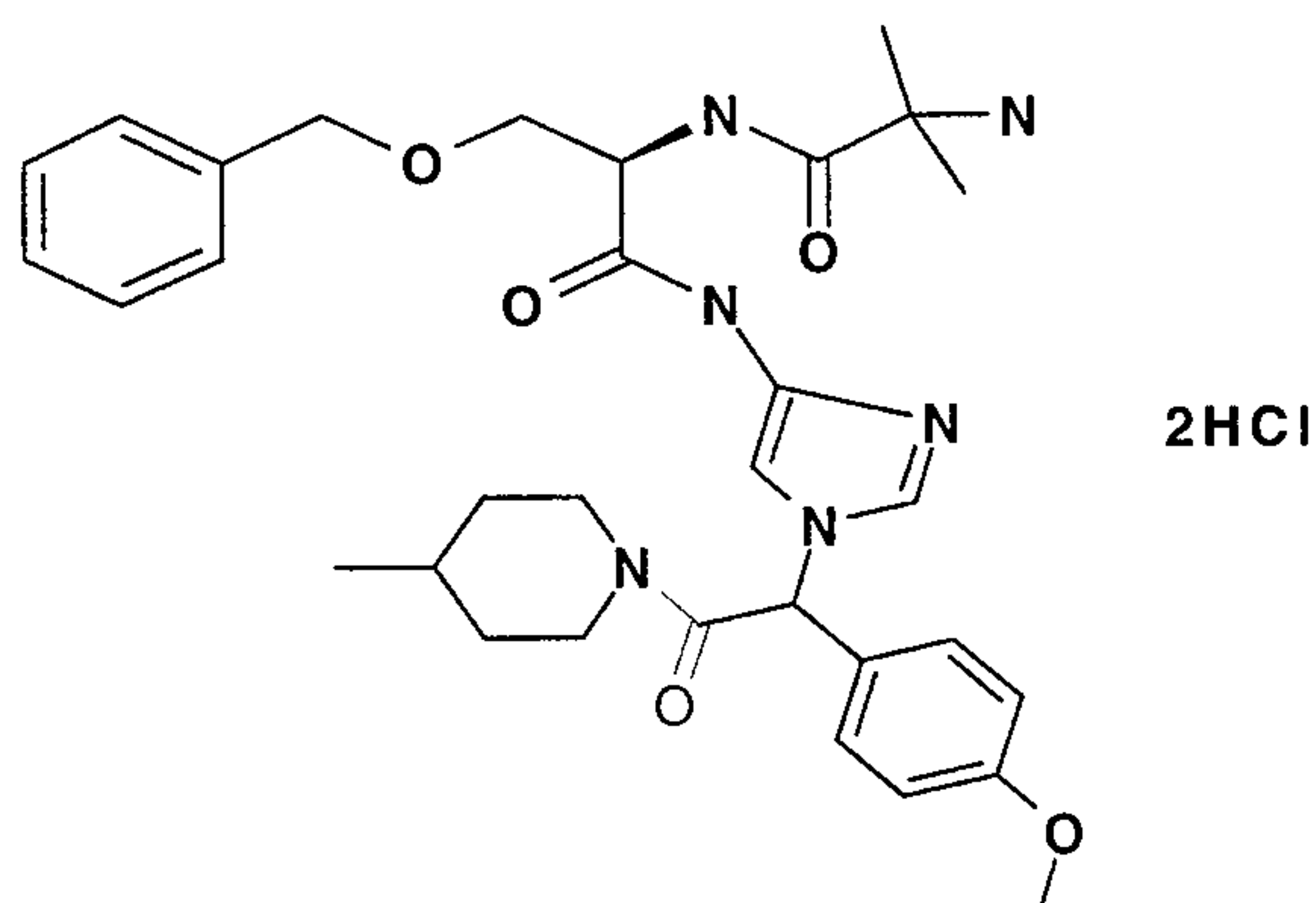
Compounds 7 and 8
