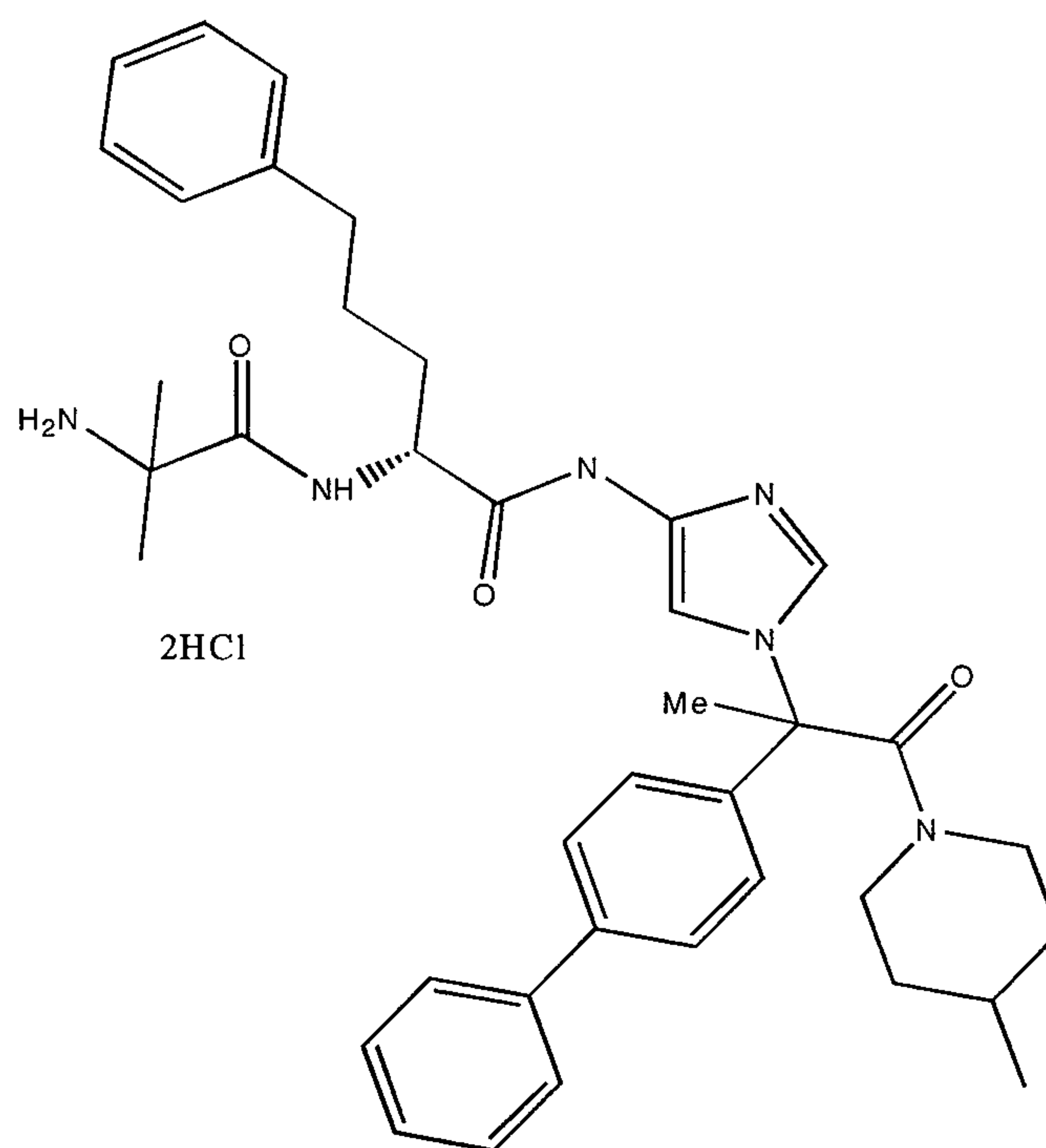
Compound 40
