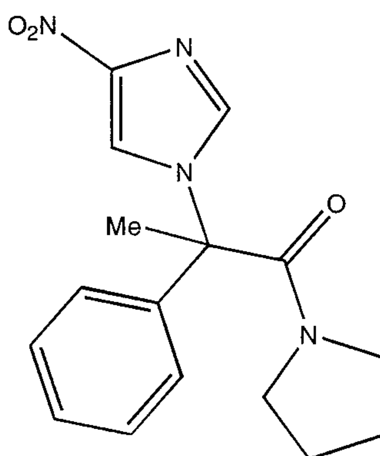
isomer 1
