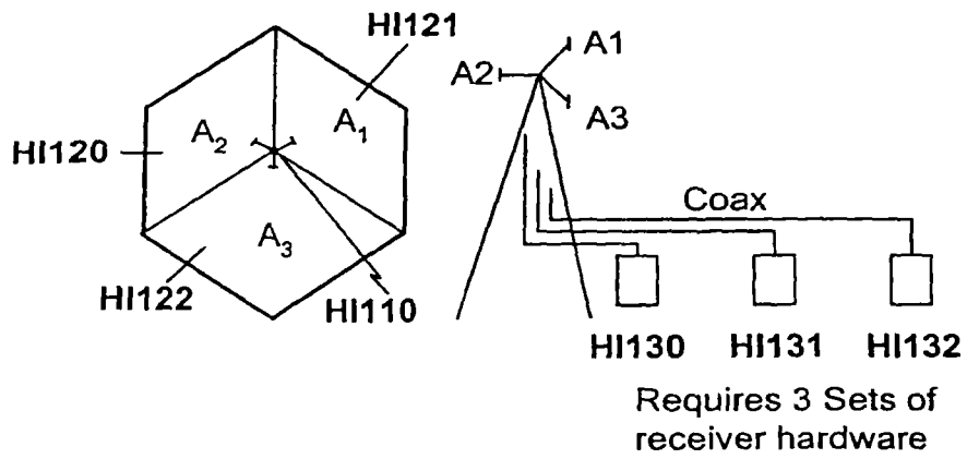
FIGURE 13 PRIOR ART
